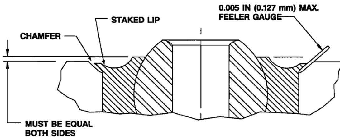
Figure 1: Example, Correctly Staked Roll Stake Bearing.
