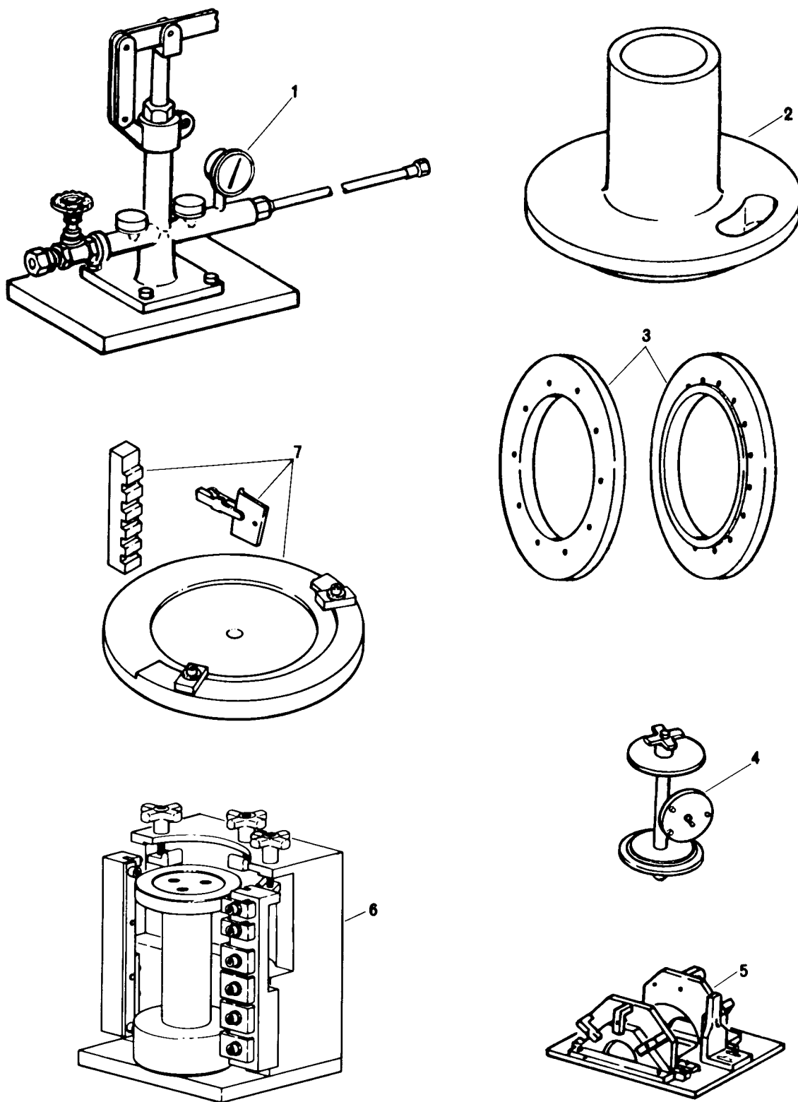
Figure E5. Special Tools
