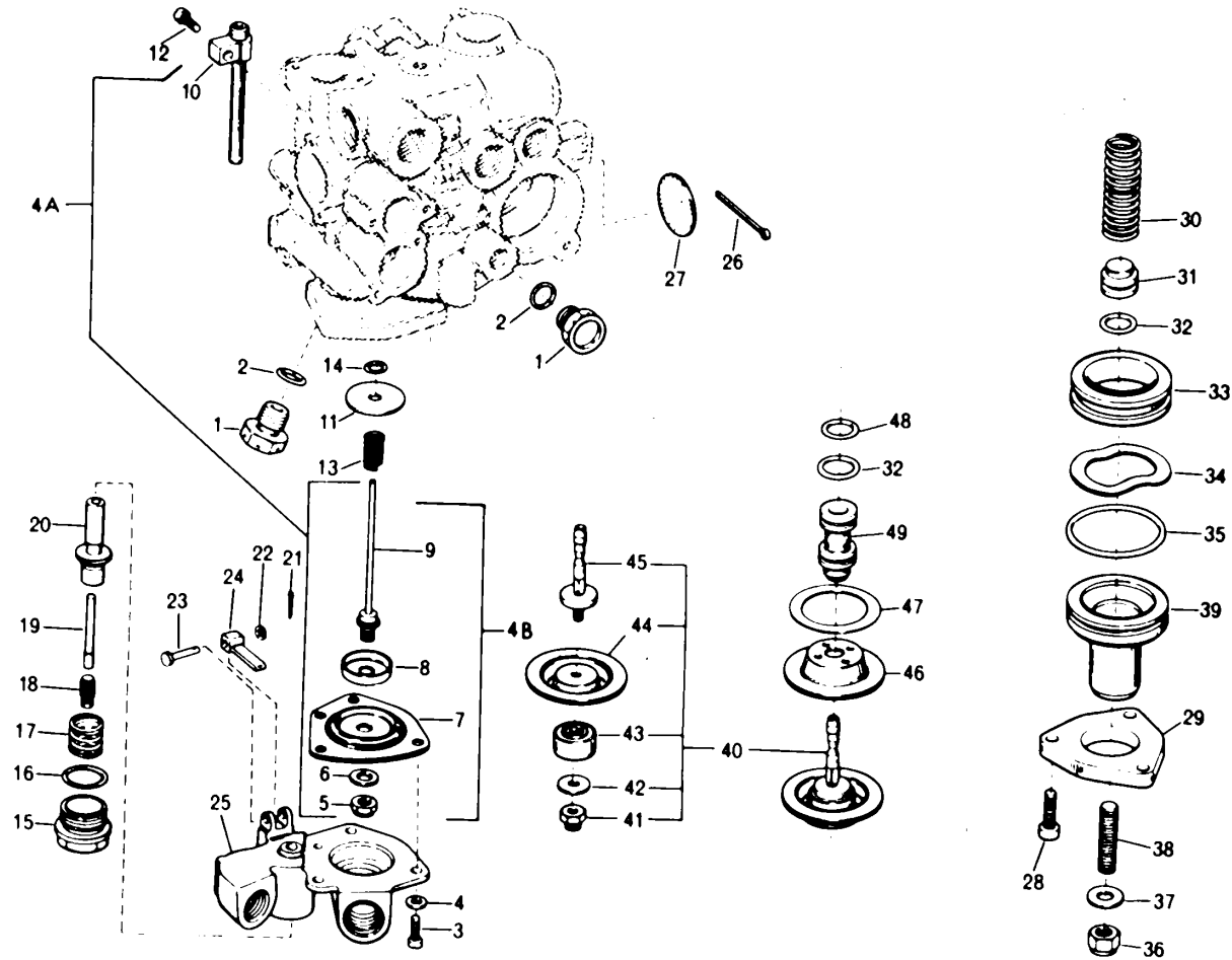
Figure 17. Fuel Control Main Flow Body (Sheet 1 of 4)
