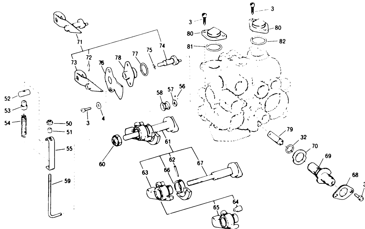
Figure 17. Fuel Control Main Body (Sheet 2 of 4)
