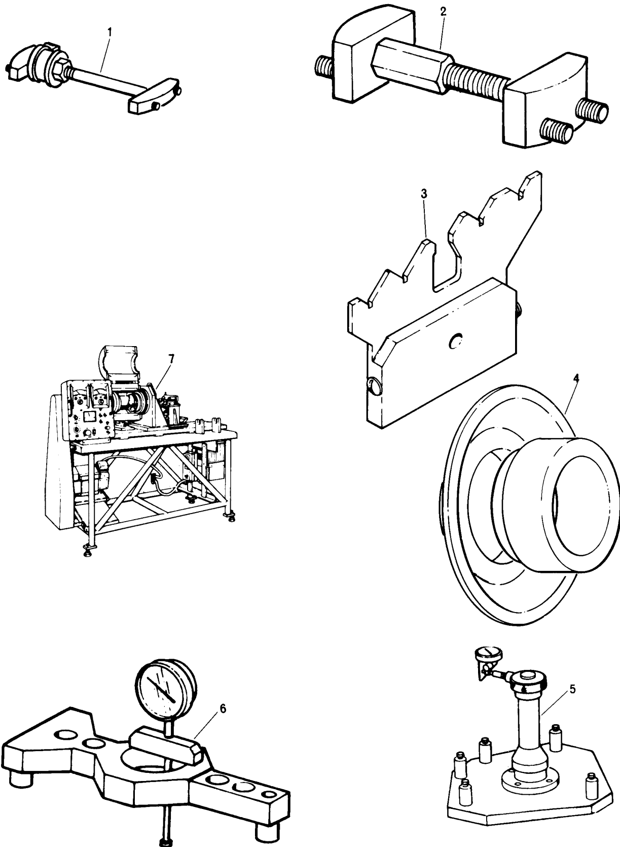
Figure E19. Special Tools
