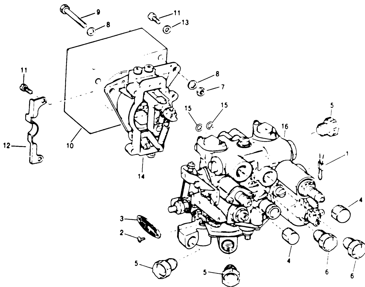
Figure 15. Turbine Main Fuel Control
