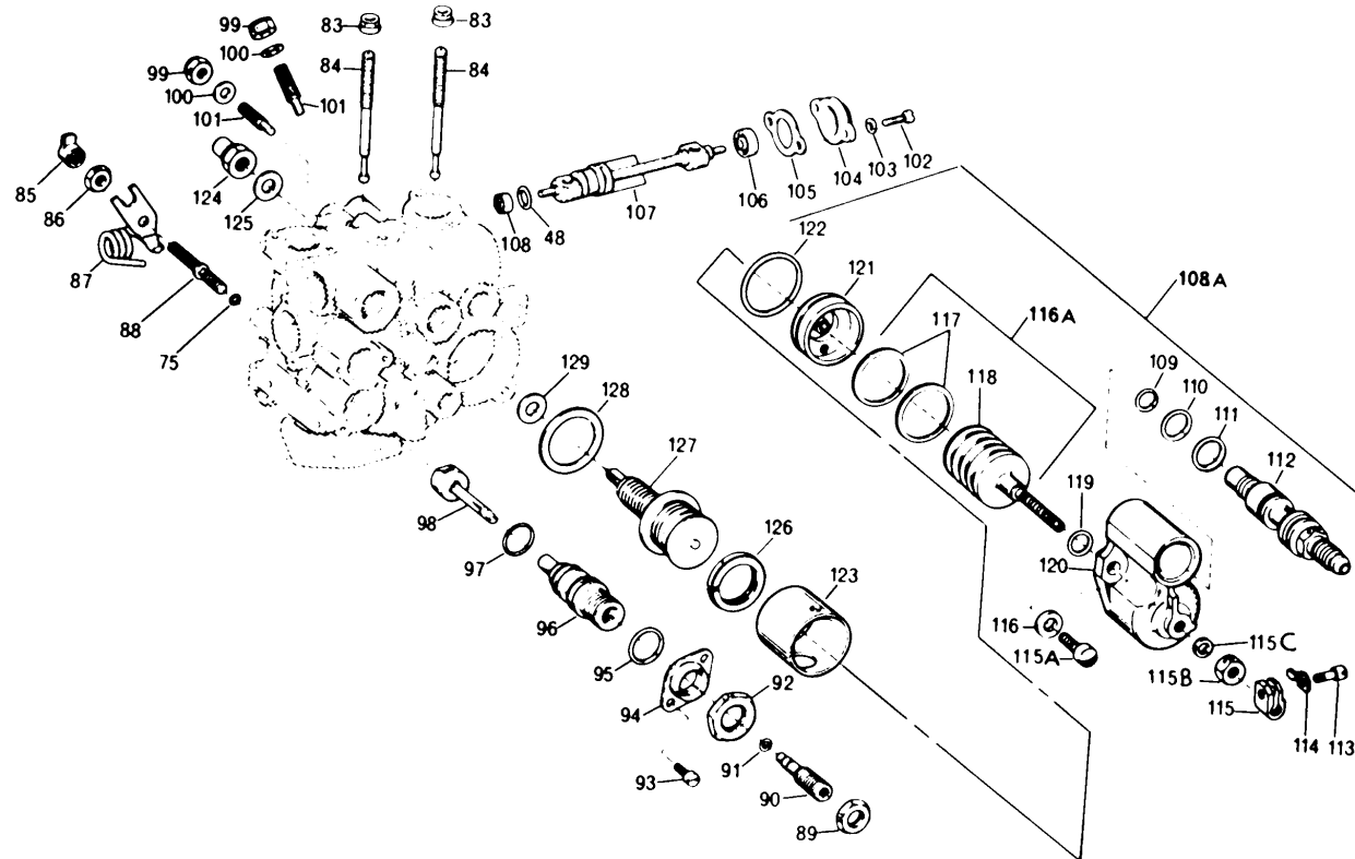
Figure 17. Fuel Control Main Flow Body (Sheet 3 of 4)
