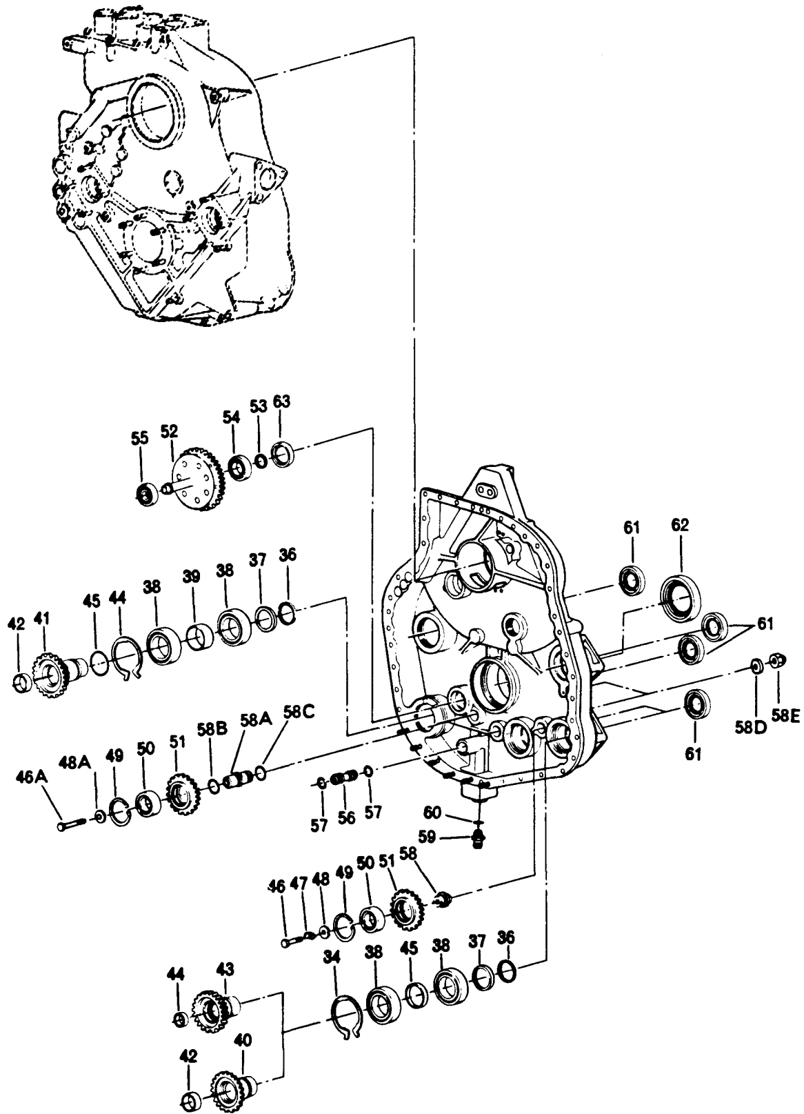
Figure 9. Accessory Drive Gearbox (Sheet 2 of 3)
