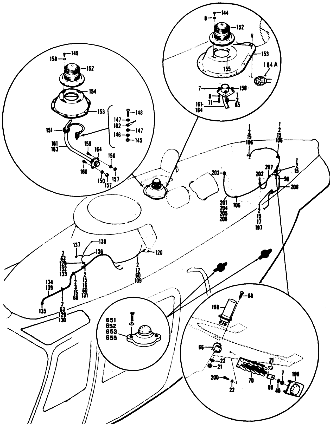
Figure 79. Electrical Installation (Sheet 3 of 12)
