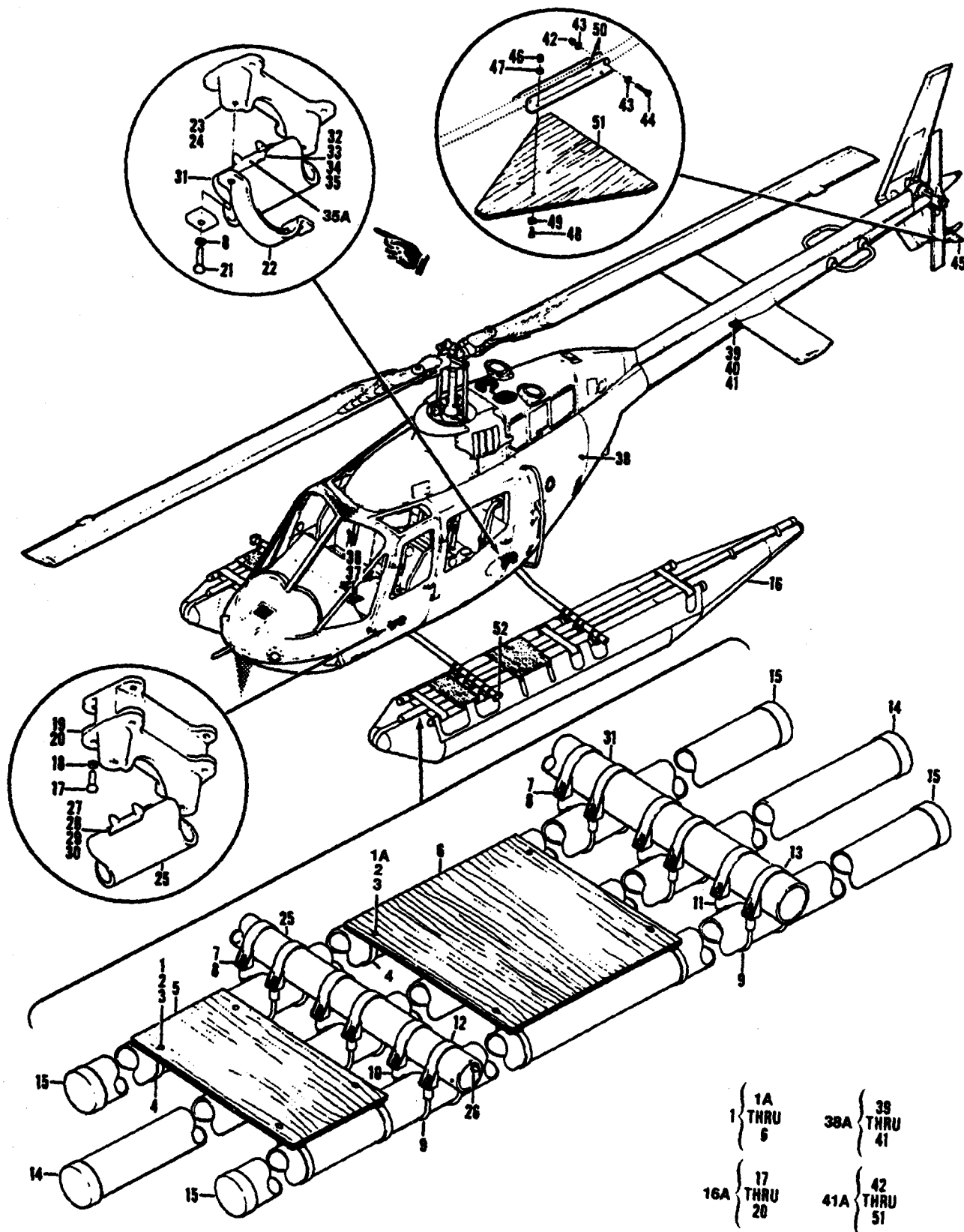
Figure 46. Kit, Float Landing Gear
