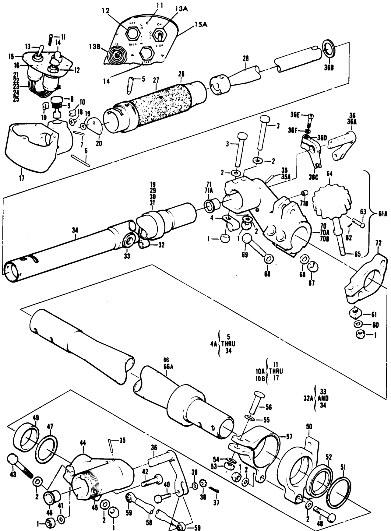
Figure 93. Jackshaft Assembly
