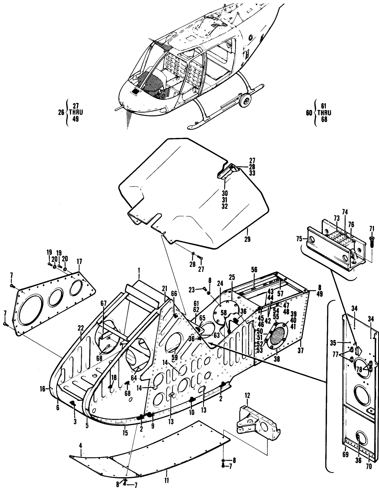
Figure 14. Console Installation
