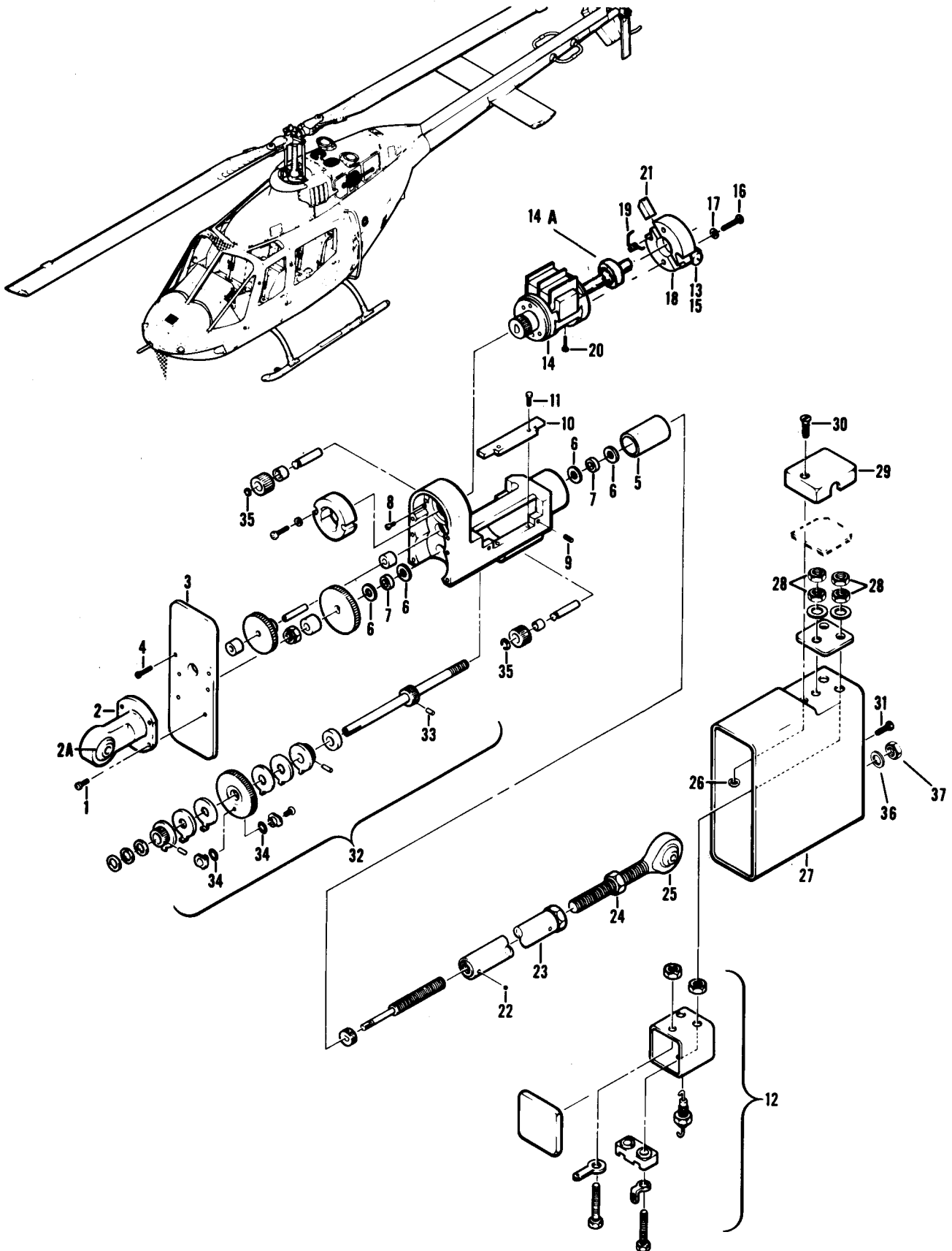
Figure 88. Electro-Mech Actuator
