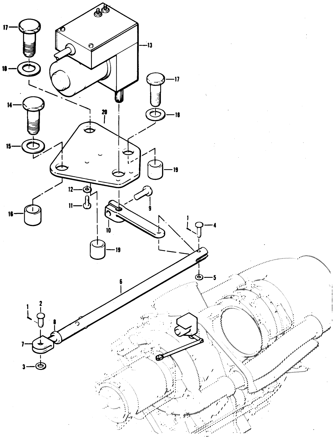
Figure 103. Control Installation, Engine Anti-icing
