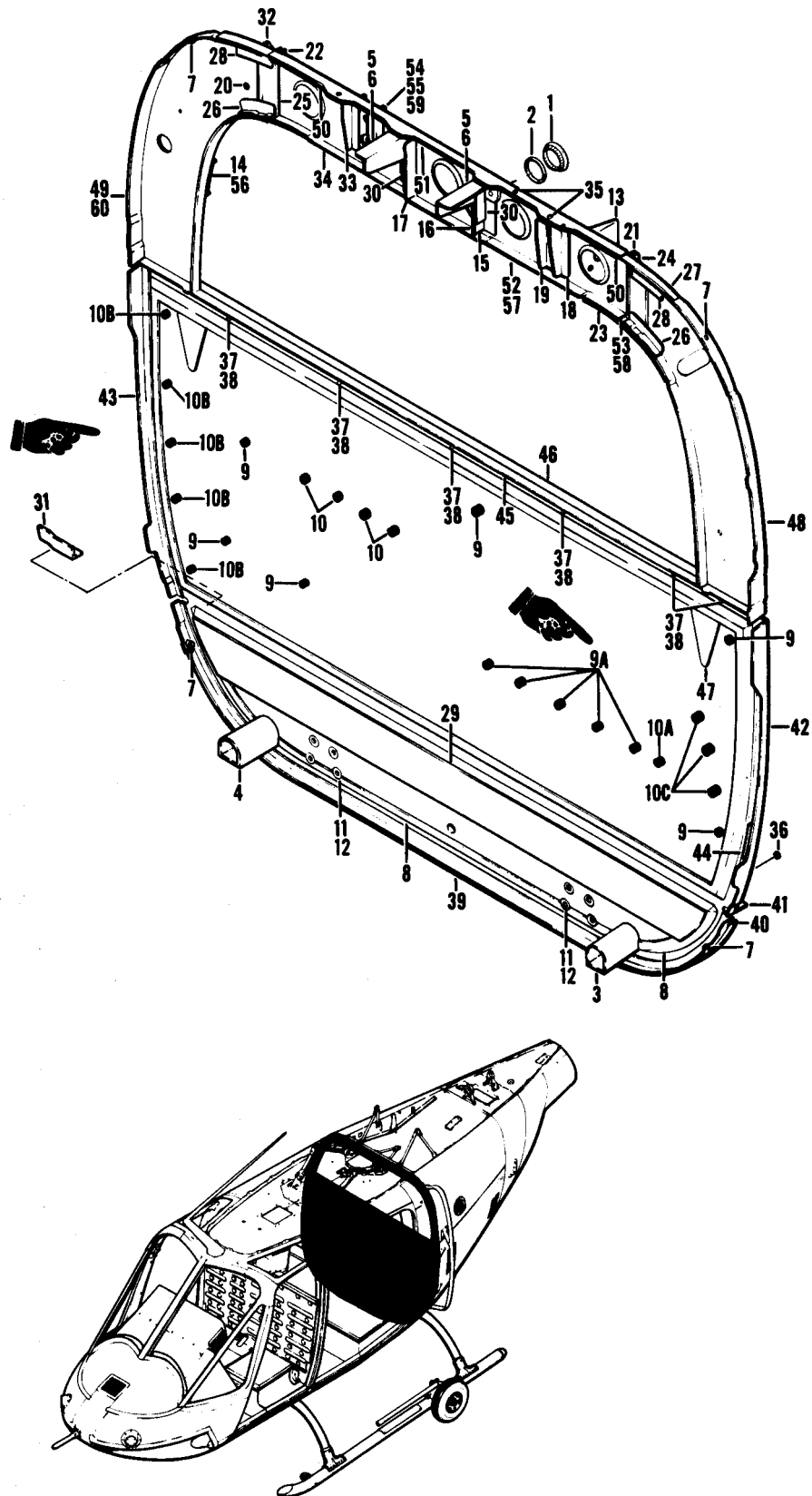
Figure 29. Bulkhead Installation
