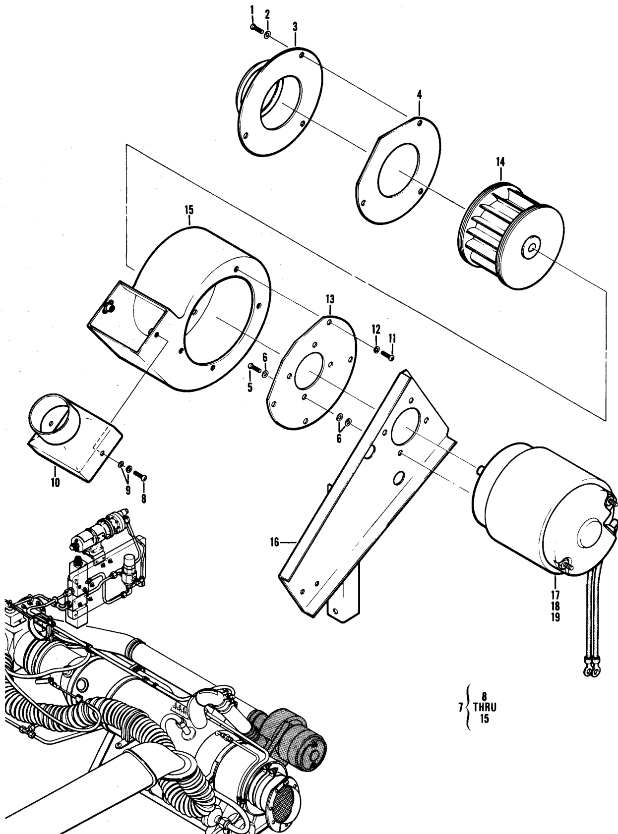
Figure 110. Blower and Motor Assembly
