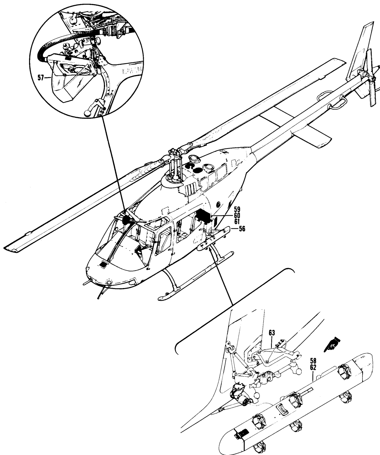
Figure 2. Helicopter Assembly (Sheet 2 of 2)
