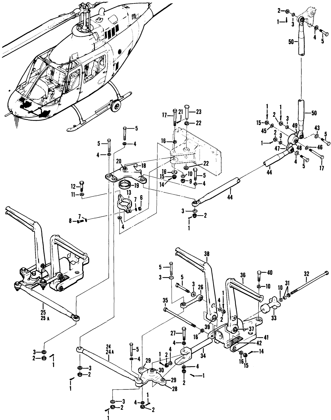
Figure 99. Controls Installation, Anti-torque (Sheet 1 of 2)
