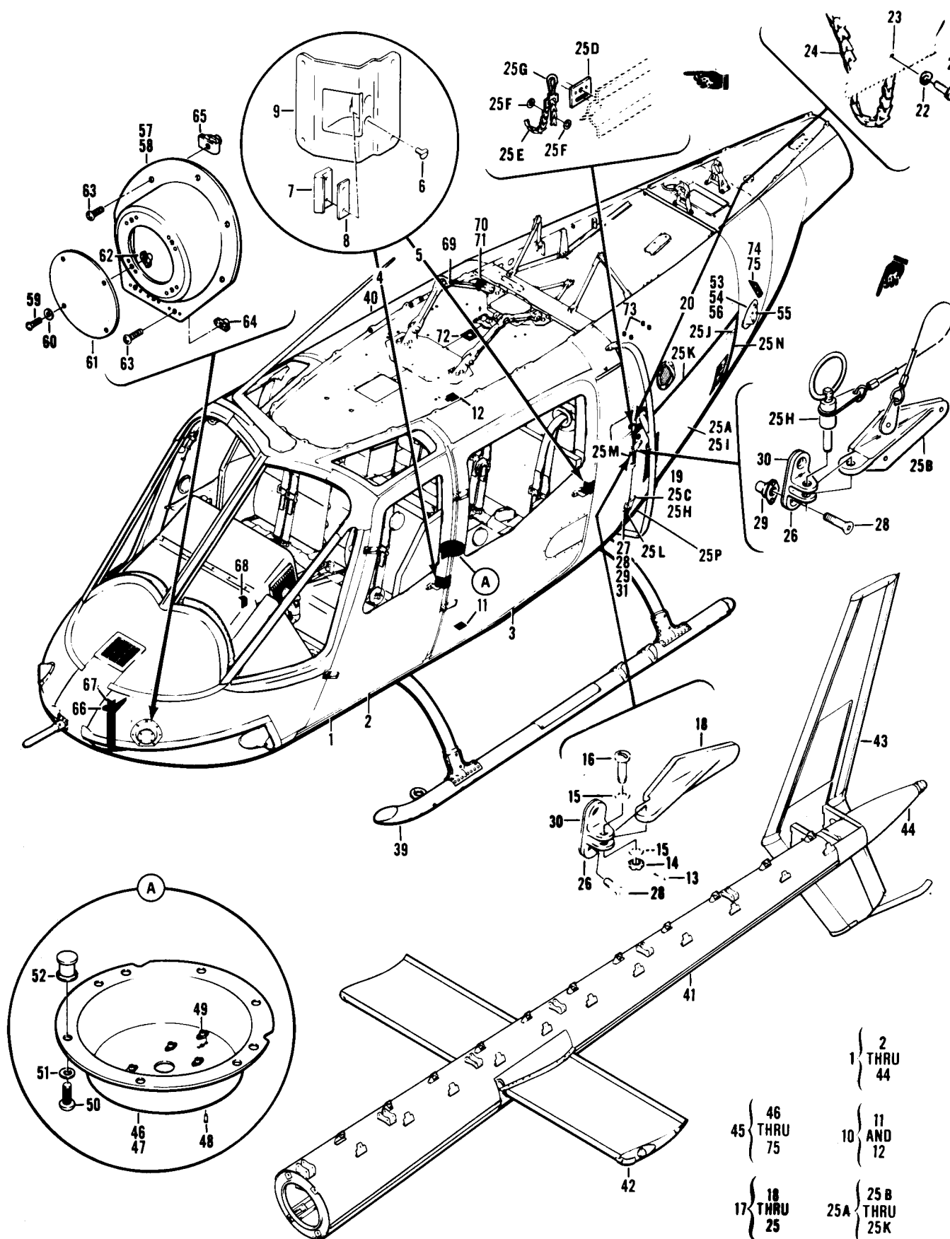
Figure 7. Forward Fuselage Assembly
