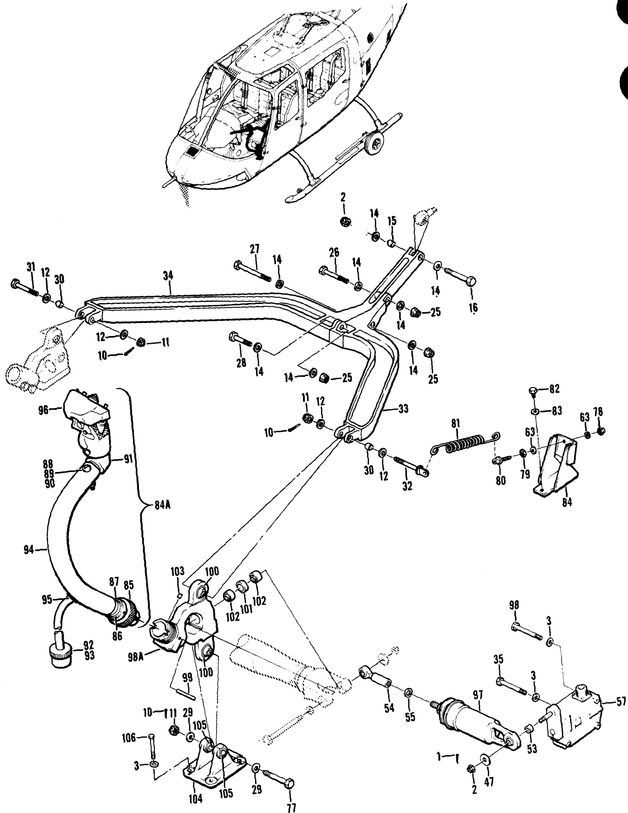
Figure 95. Control Installation, Cyclic (Sheet 2 of 2)
