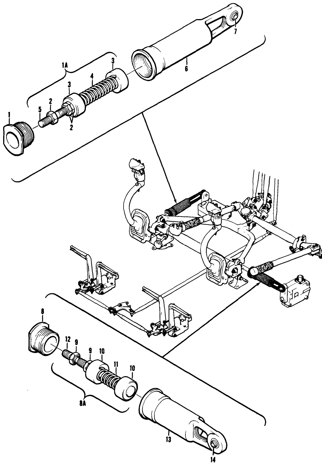
Figure 97. Force Gradient Assembly
