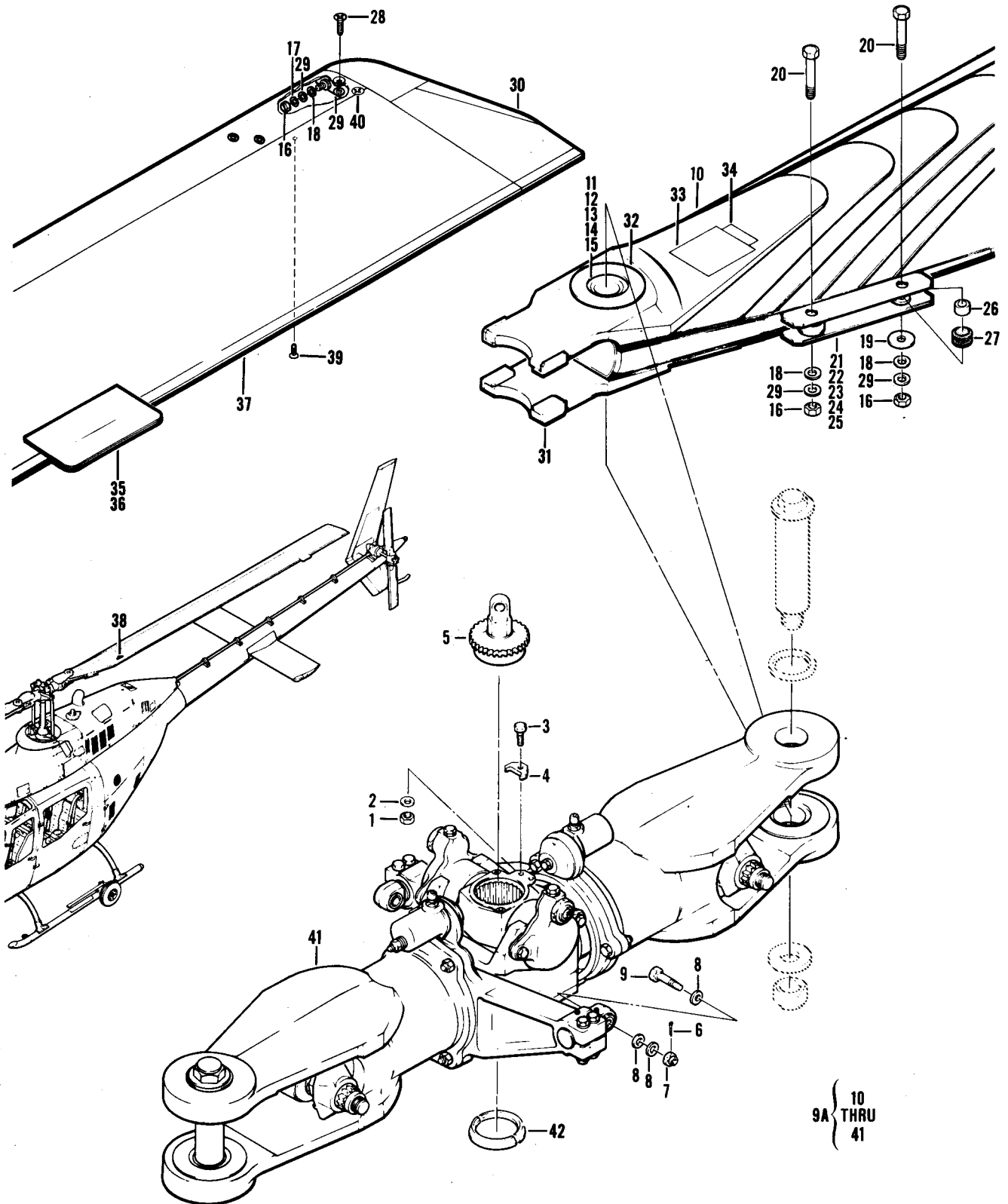
Figure 57. Main Rotor Hub and Blade Installation
