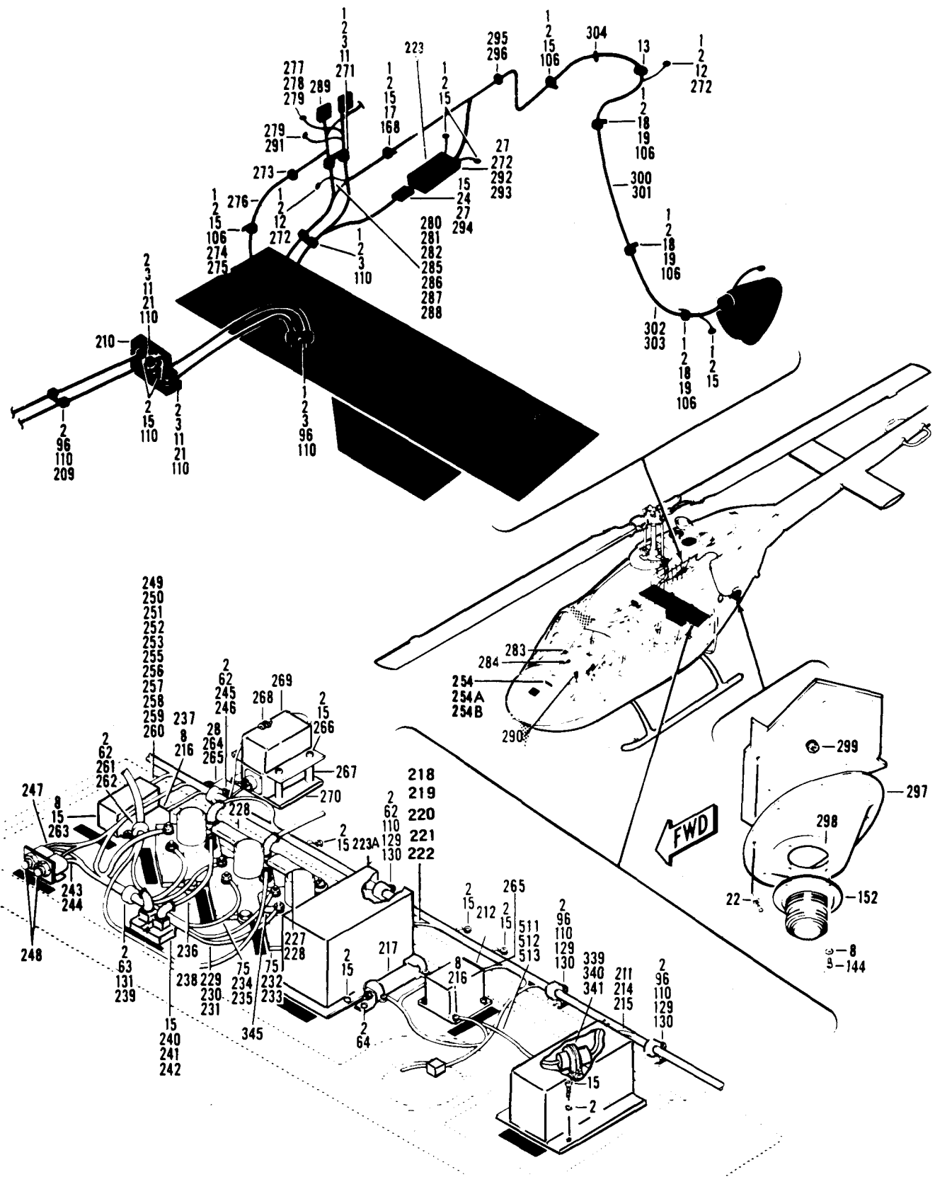
Figure 79. Electrical Installation (Sheet 5 of 12)
