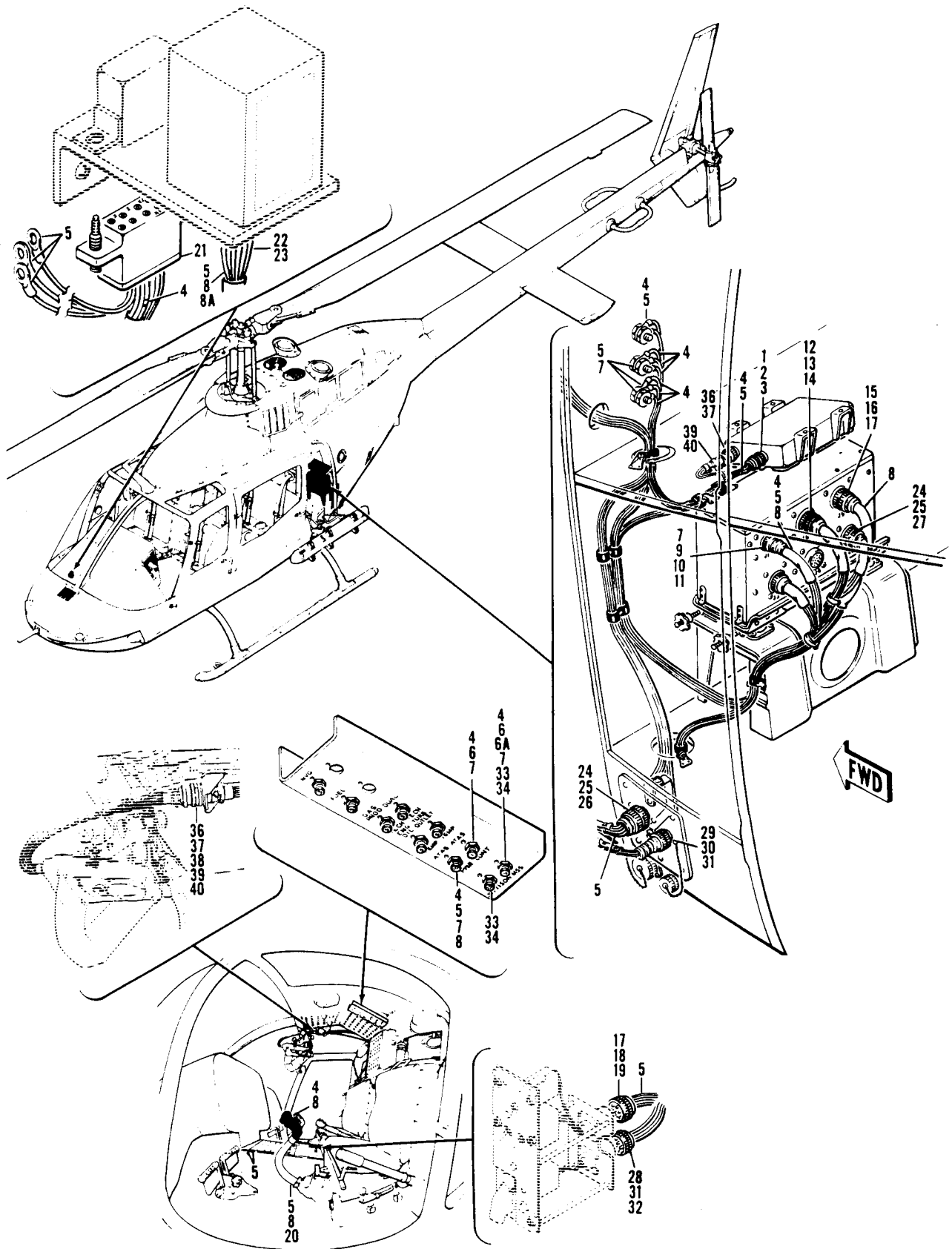
Figure 89C. Cable Assembly
