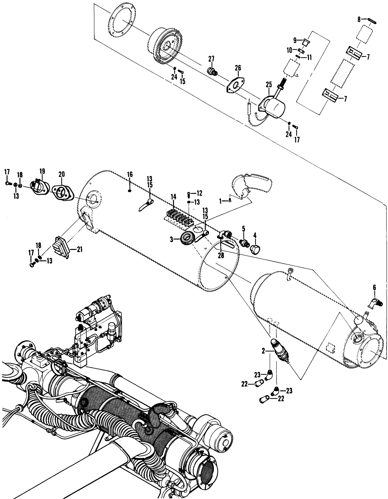
Figure 109. Heater Assy
