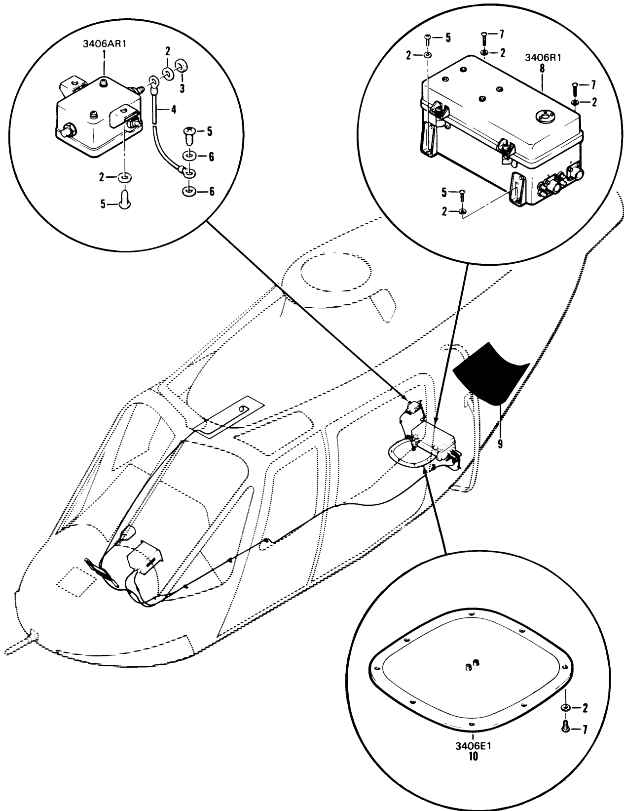
Figure 32. Direction Finder Set AN/ARN-89 (Sheet 1 of 2).
