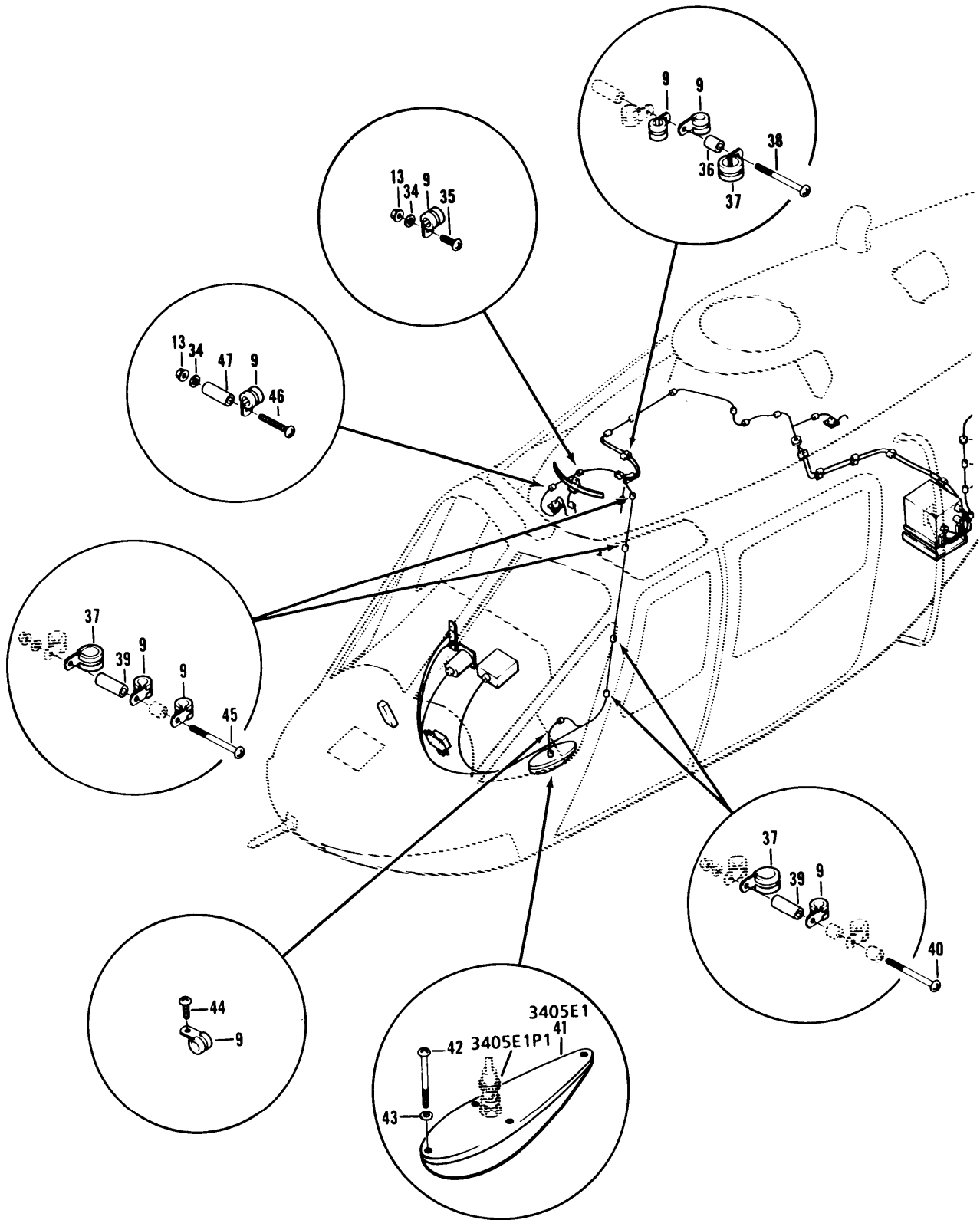
Figure 49. Civil Navigation System AN/ARN-123(V)/1 (C Model Only (Sheet 2 of 3).
