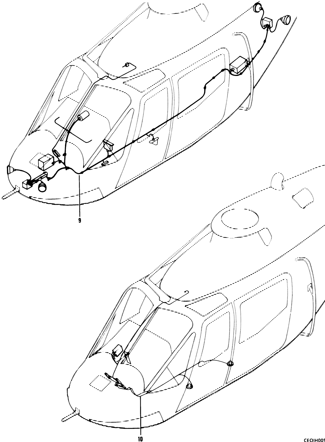
Figure 1. OH-58A/C Electronics Configuration (Sheet 5 of 7).
