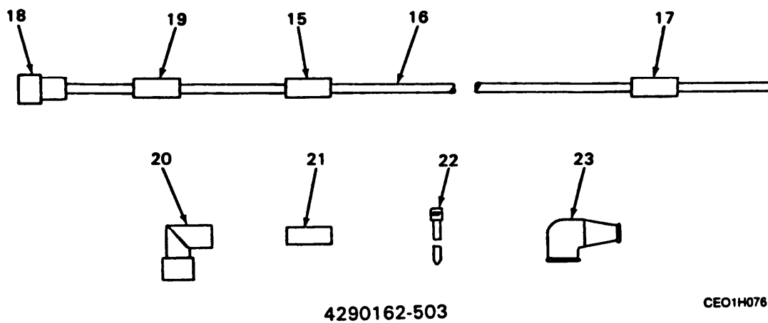
Figure 22. Cable Assembly, Coax 4290162-501, 4290162-502, 4290162-503, 4290162-504, 4290162-505, 4290162-506 (Sheet 1 of 2)
