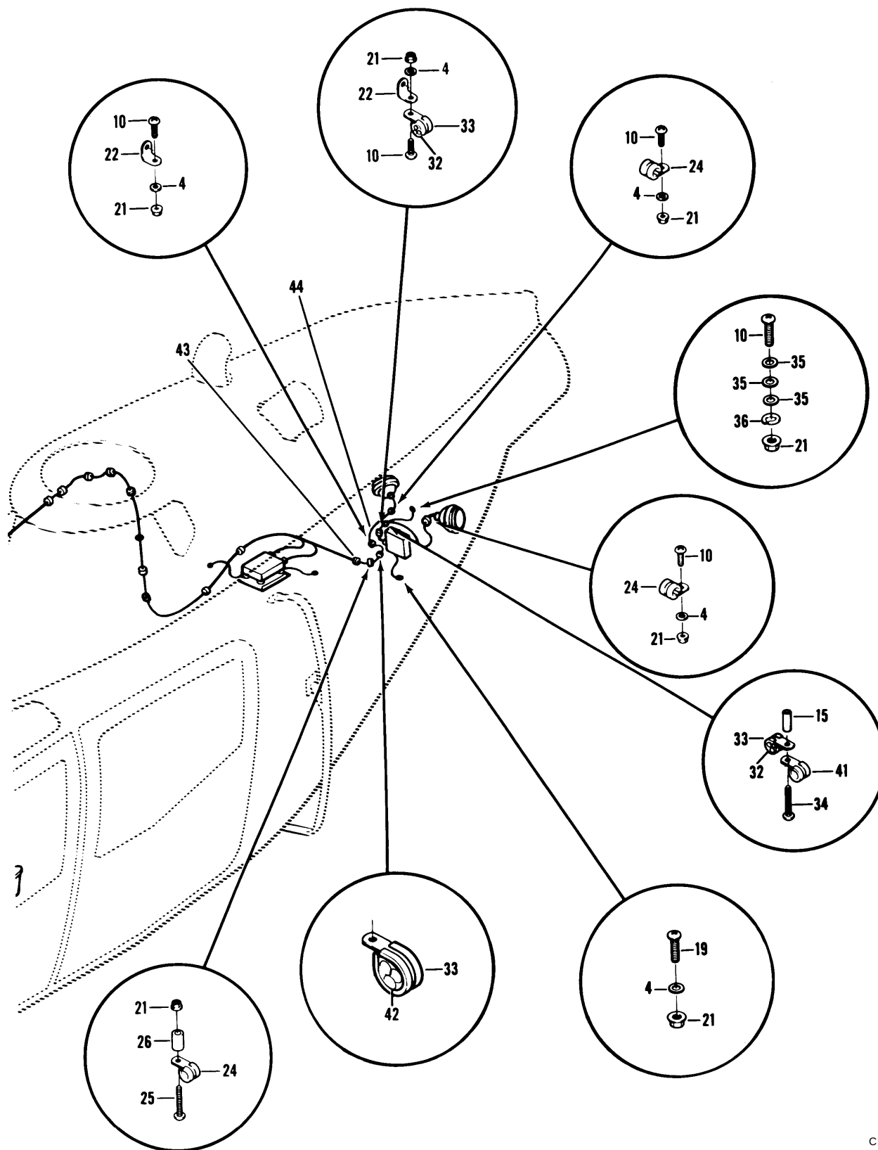
Figure 47. Detecting Set, Radar Signal AN/APR-39(V)1 (C Model Only) (Sheet 4 of 5).
