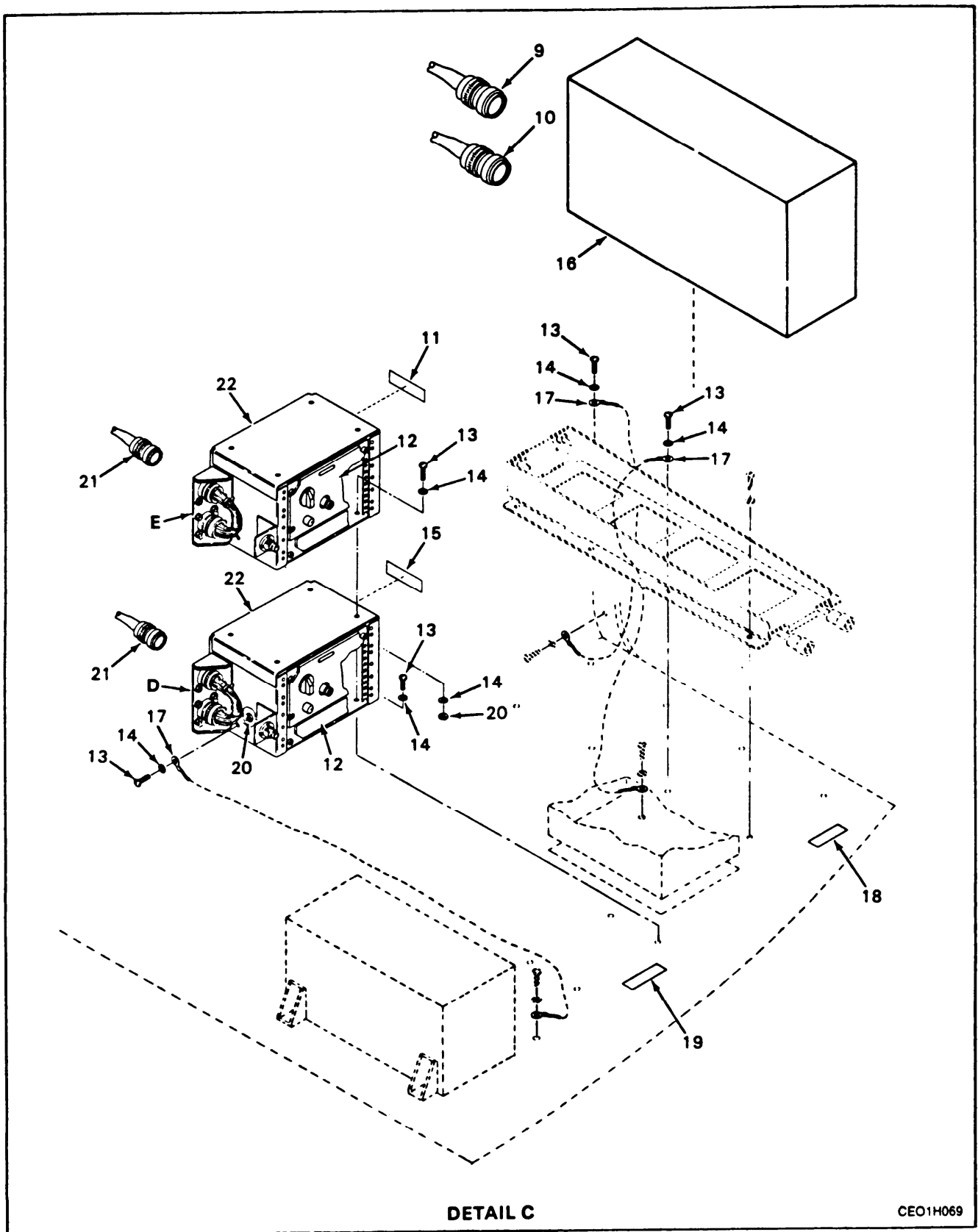
Figure 13. VHF-FM Communications System with SINCGARS (Sheet 3 of 6)
