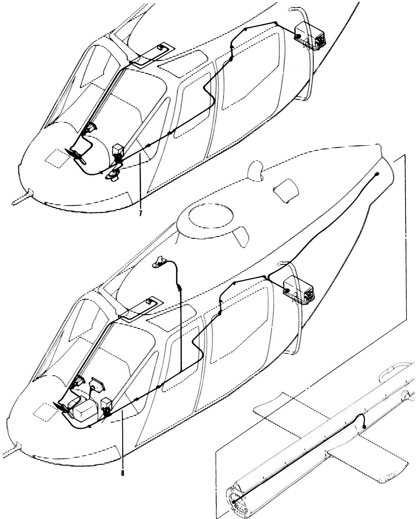
Figure 1. OH-58A/C Electronics Configuration (Sheet 4 of 7).
