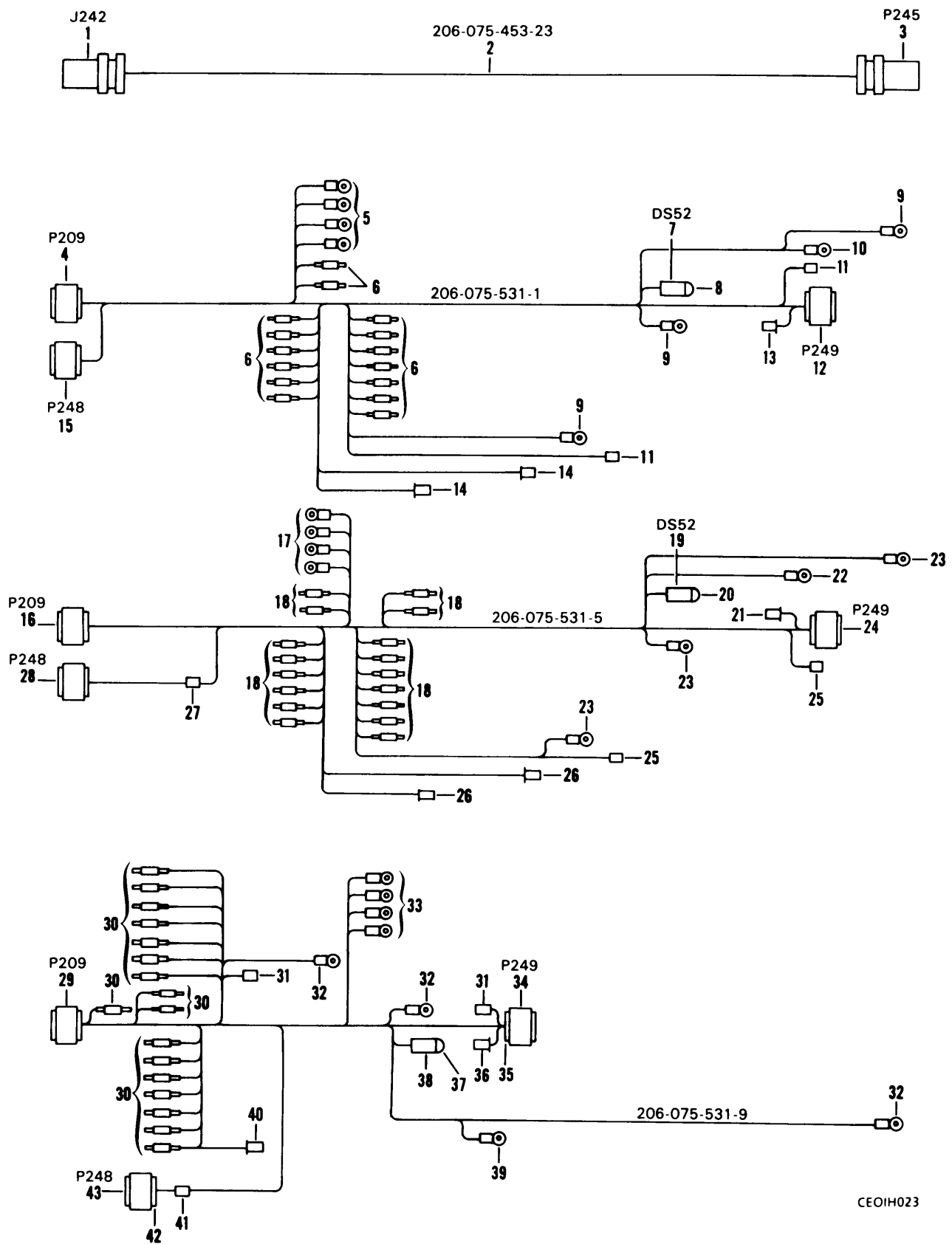
Figure 18. Cable Assemblies (206-075-453-23, 206-075-531-1, 206-075-531-5, 206-075-531-9).
