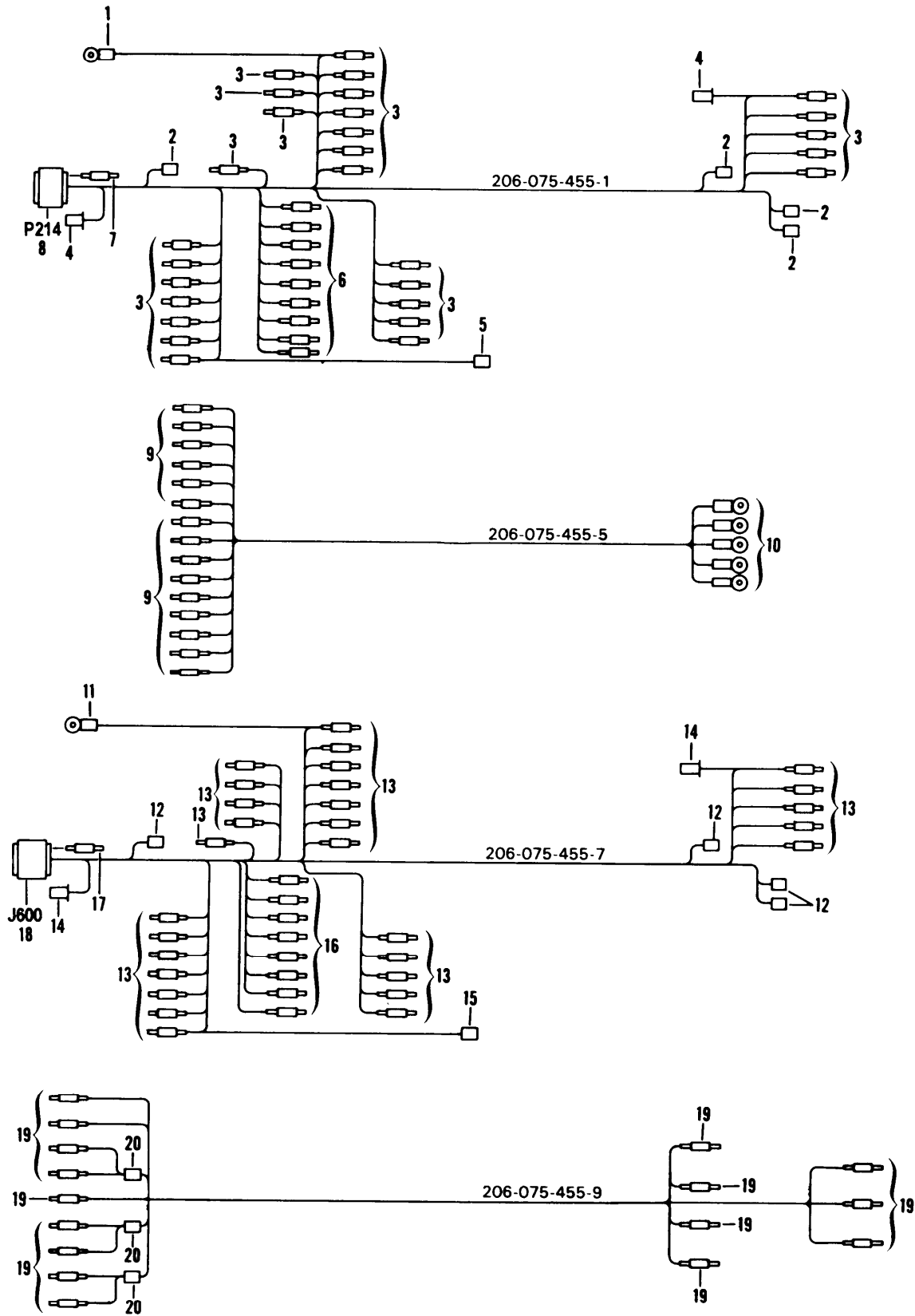
Figure 7. Cable Assemblies (206-075-455-1, 206-075-455-5, 206-075-455-7, 206-075-455-9).
