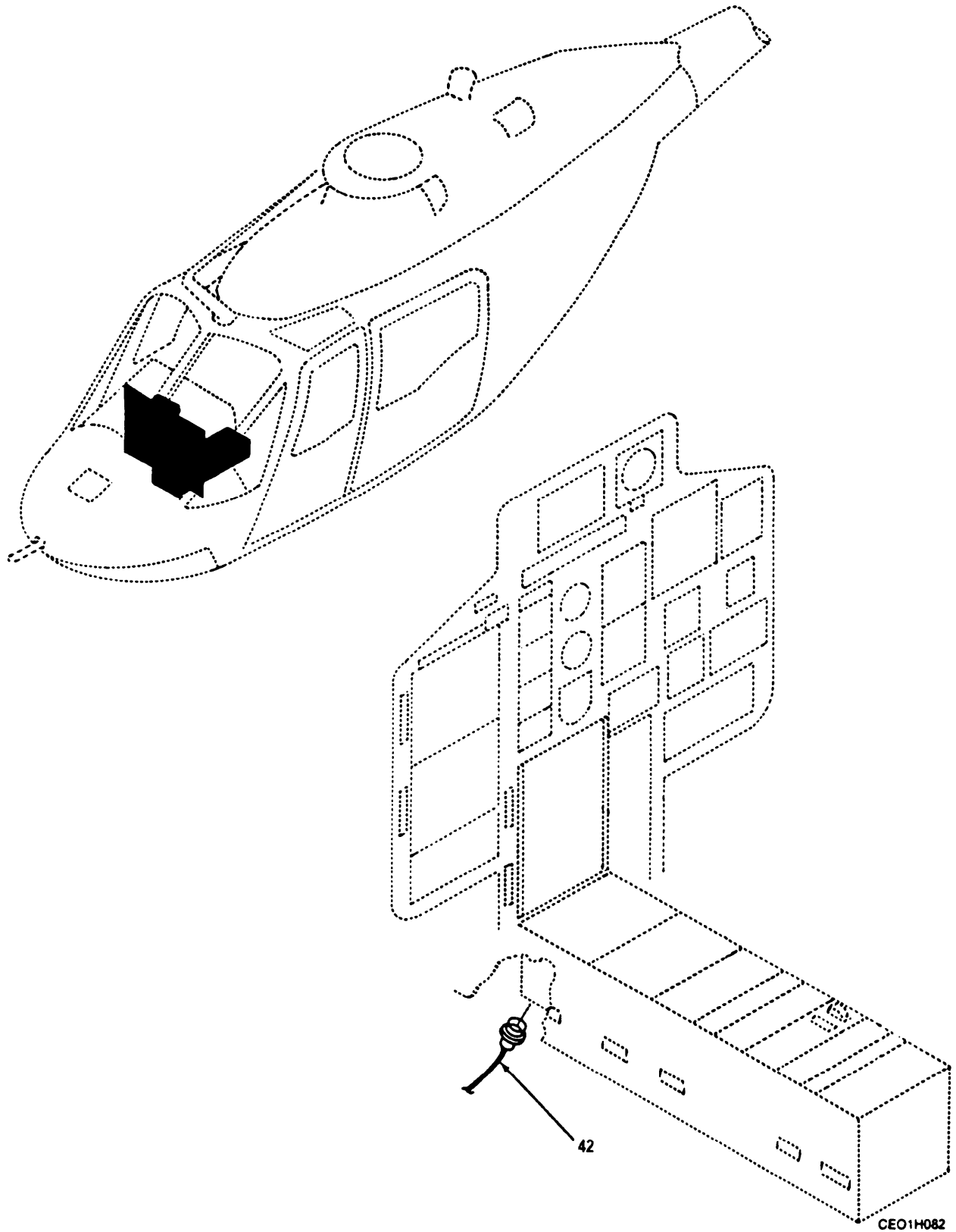
Figure 40. Transponder (IFF) System AN/APX-72 (A Model Only) (Sheet 3 of 3).
