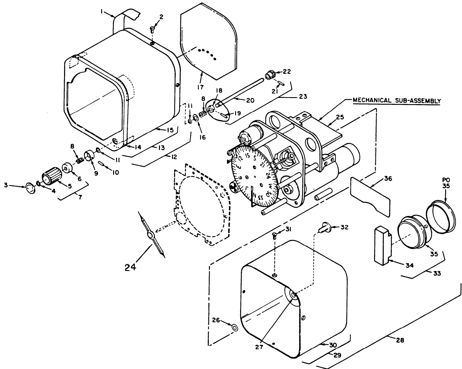
Figure 37. Indicator, Heading and Bearing ID-1351NA.
