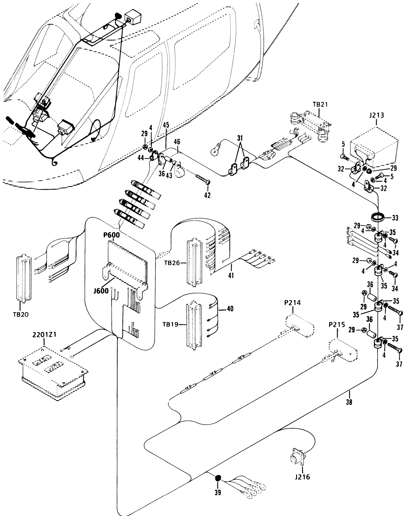
Figure2. intercom System (Sheet 20f3).
