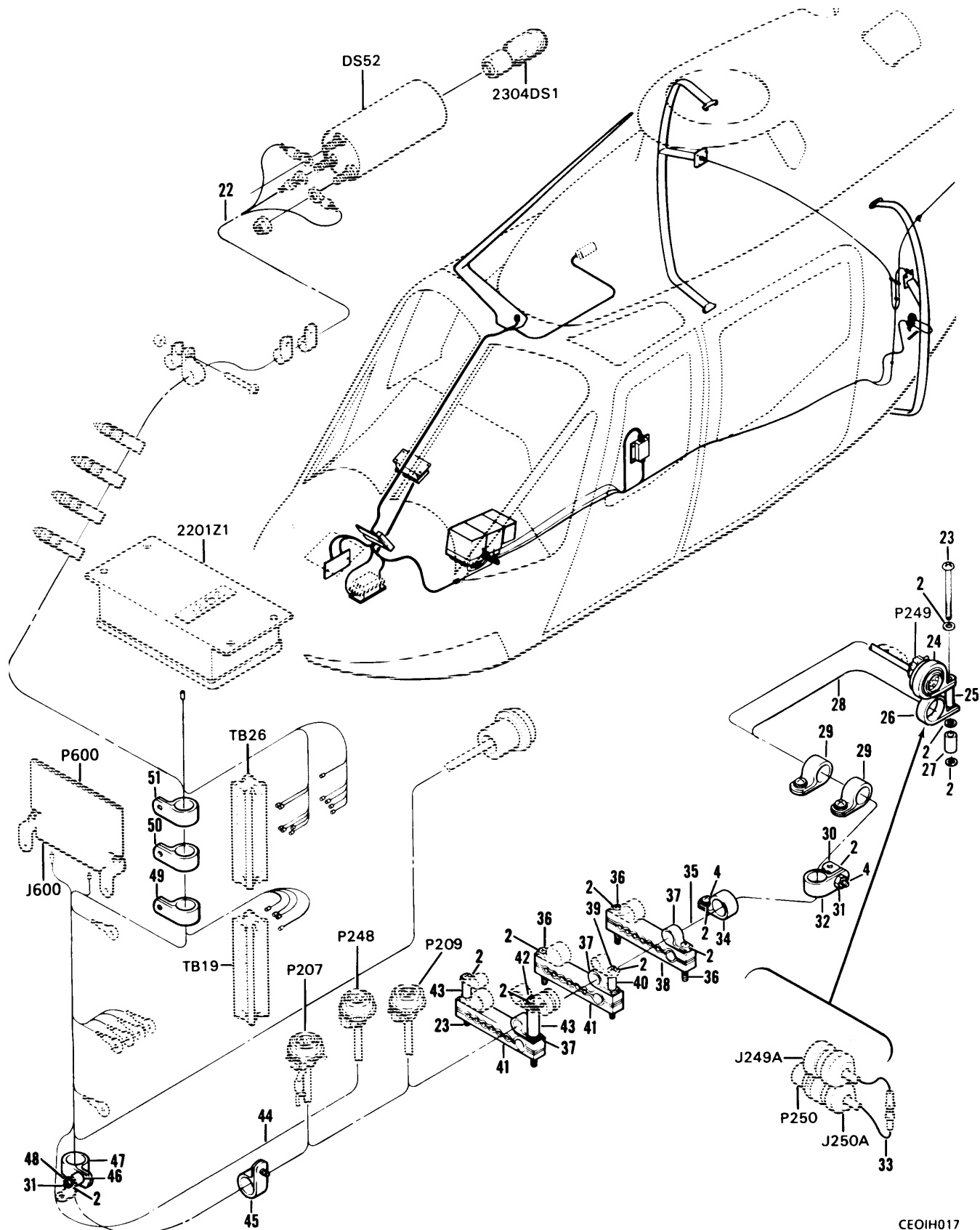
Figure 11. VHF-FM Communications System (Sheet 2 of 3).
