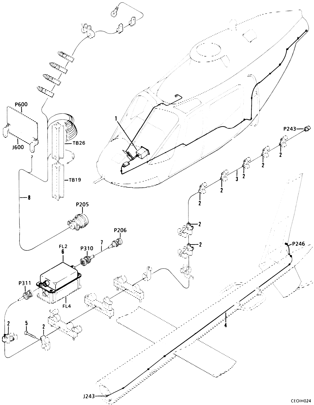
Figure 26. VHF-AM Communications System.
