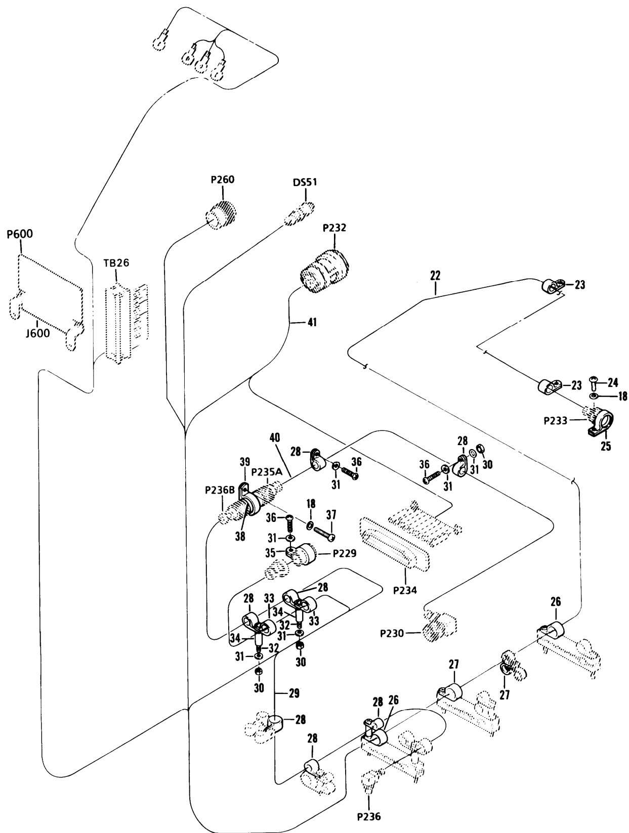
Figure 40. Transponder (IFF) System AN/APX-72 (A Model Only) (Sheet 2 of 3).
