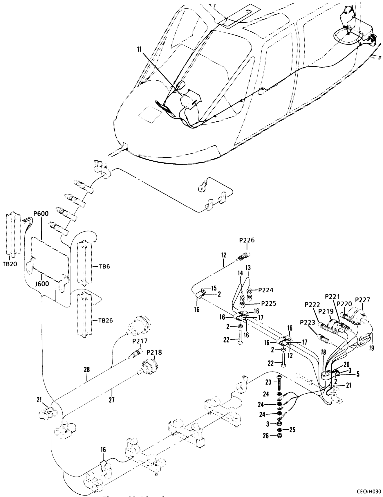
Figure 32. Direction Finder Set AN/ARN-89 (Sheet 2 of 2).
