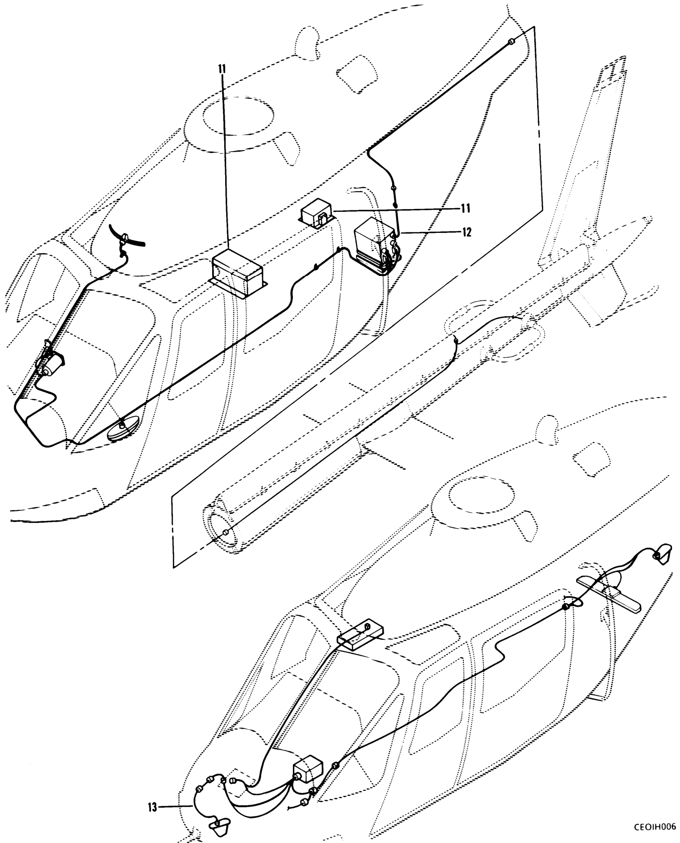
Figure 1. OH-58A/C Electronics Configuration (Sheet 6 of 7).
