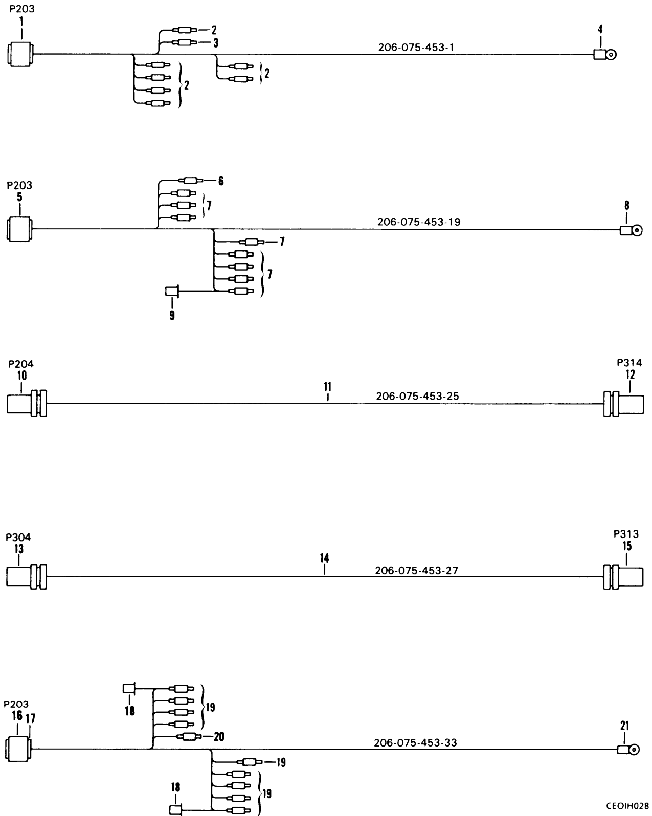
Figure 30. Cable Assemblies (206-075-453-1, 206-075-453- 19,206-075-453-25, 206-075-453-27, 206-075-453-33) .
