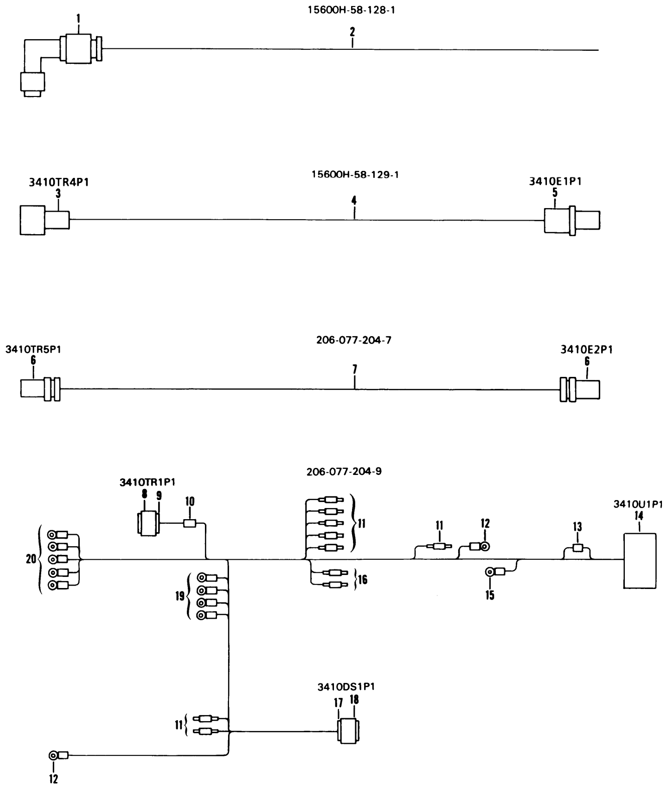
Figure 44. Cable Assemblies (15600H-58-128-1, 15600H-58-129-1, 206-077-204-7, 206-077-204-9).
