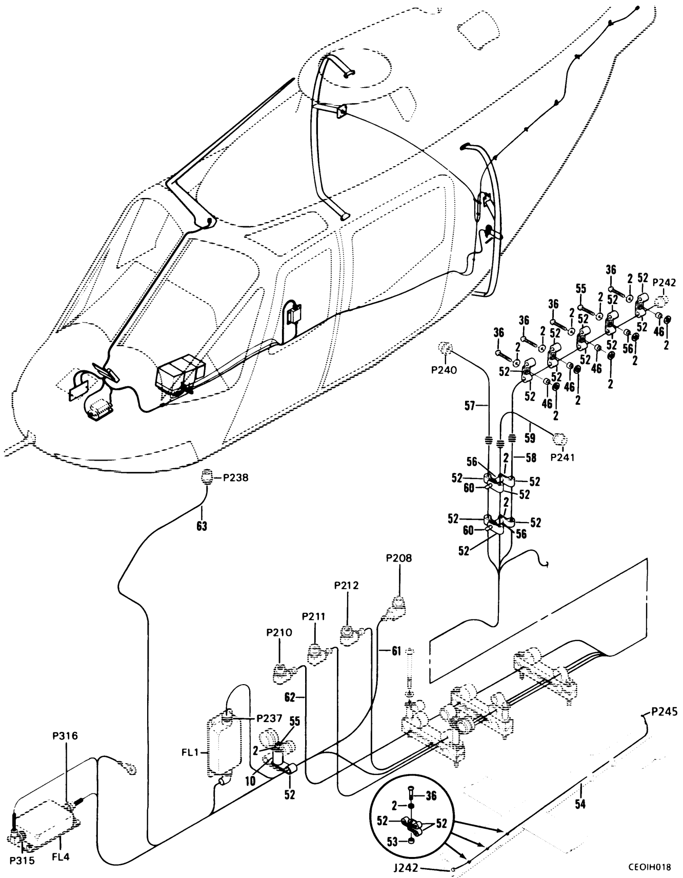
Figure 11. VHF-FM Communications System (Sheet 3 of 3).
