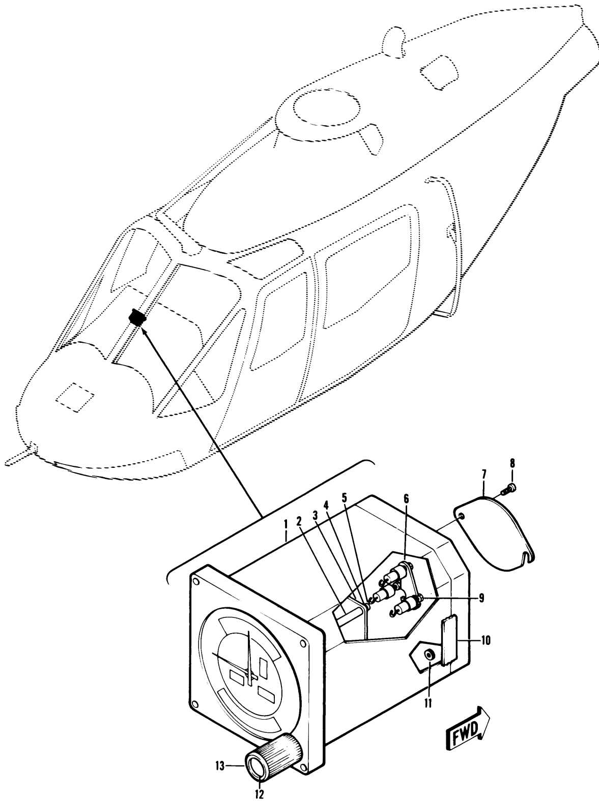
Figure 50. Indicator, Course Deviation ID-1347/ARN-82 (206-075-716-1).
