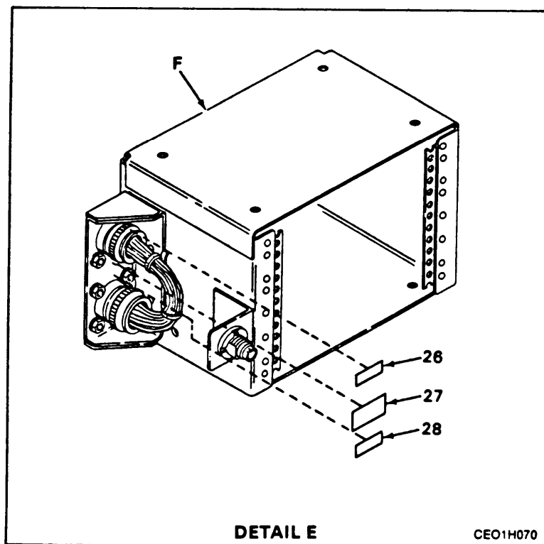
Figure 13. VHF-FM Communications System with SINCGARS (Sheet 4 of 6)
