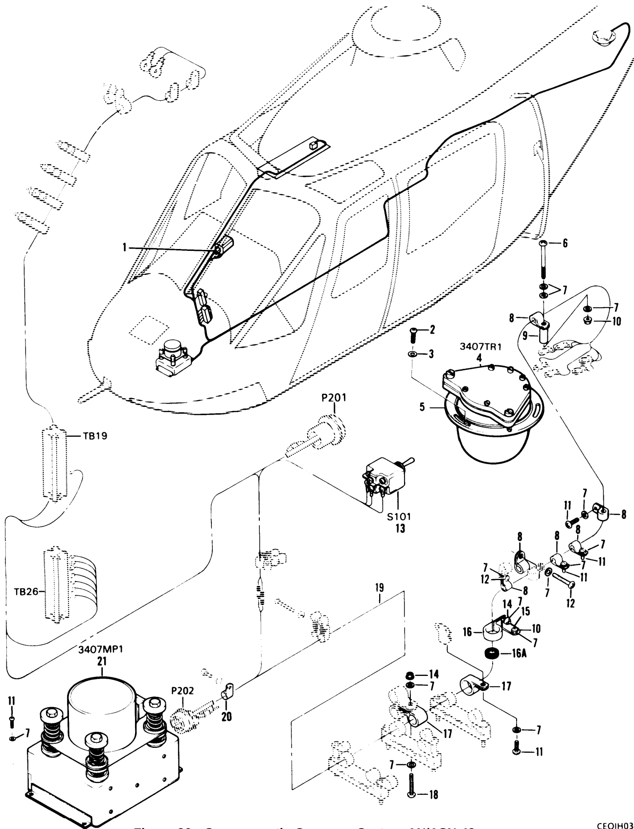
Figure 36. Gyromagnetic Compass System AN/ASN-43.
