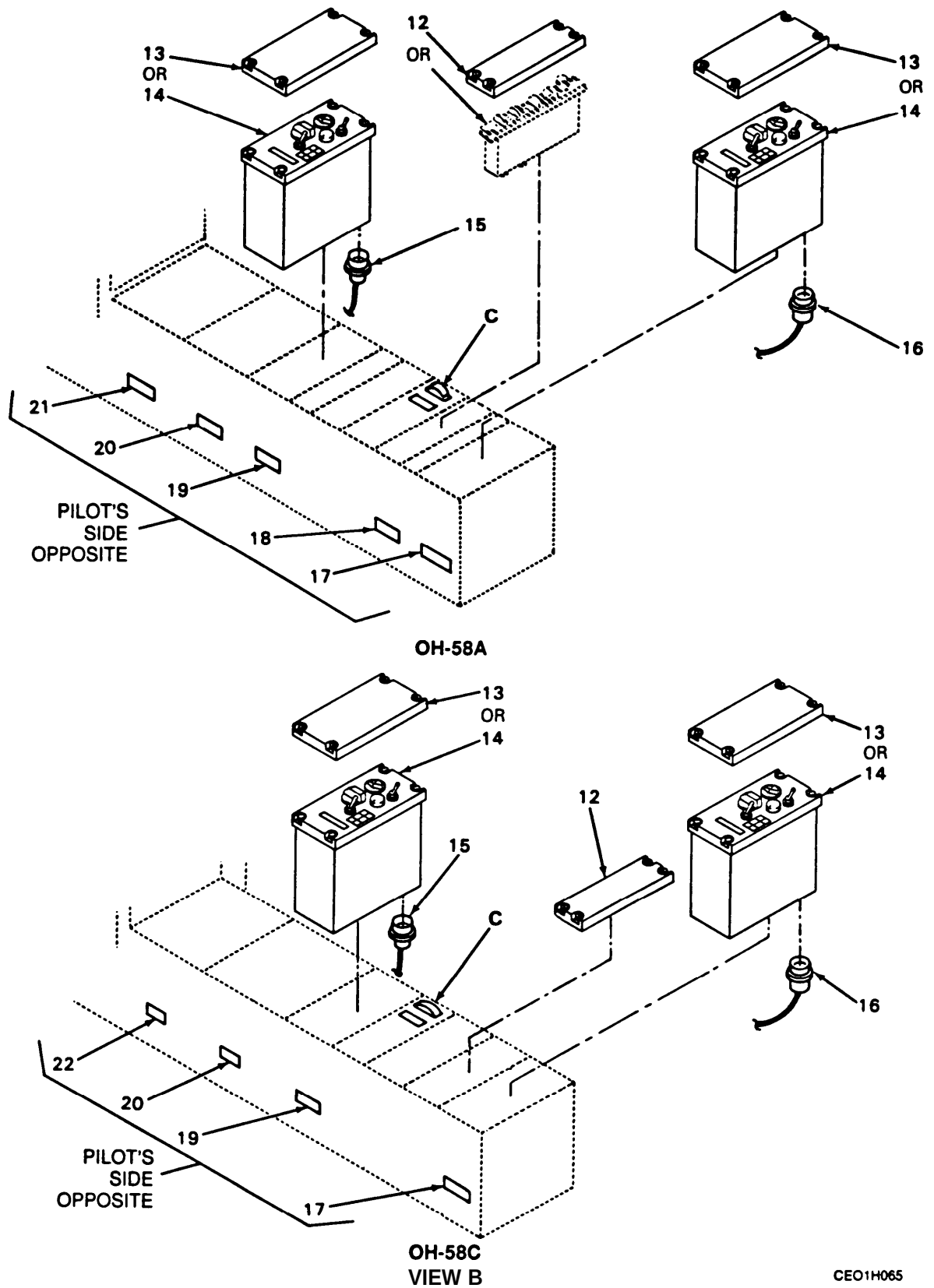
Figure 12. VHF-FM Communications System with SINCGARS, Console (Sheet 3 of 4)
