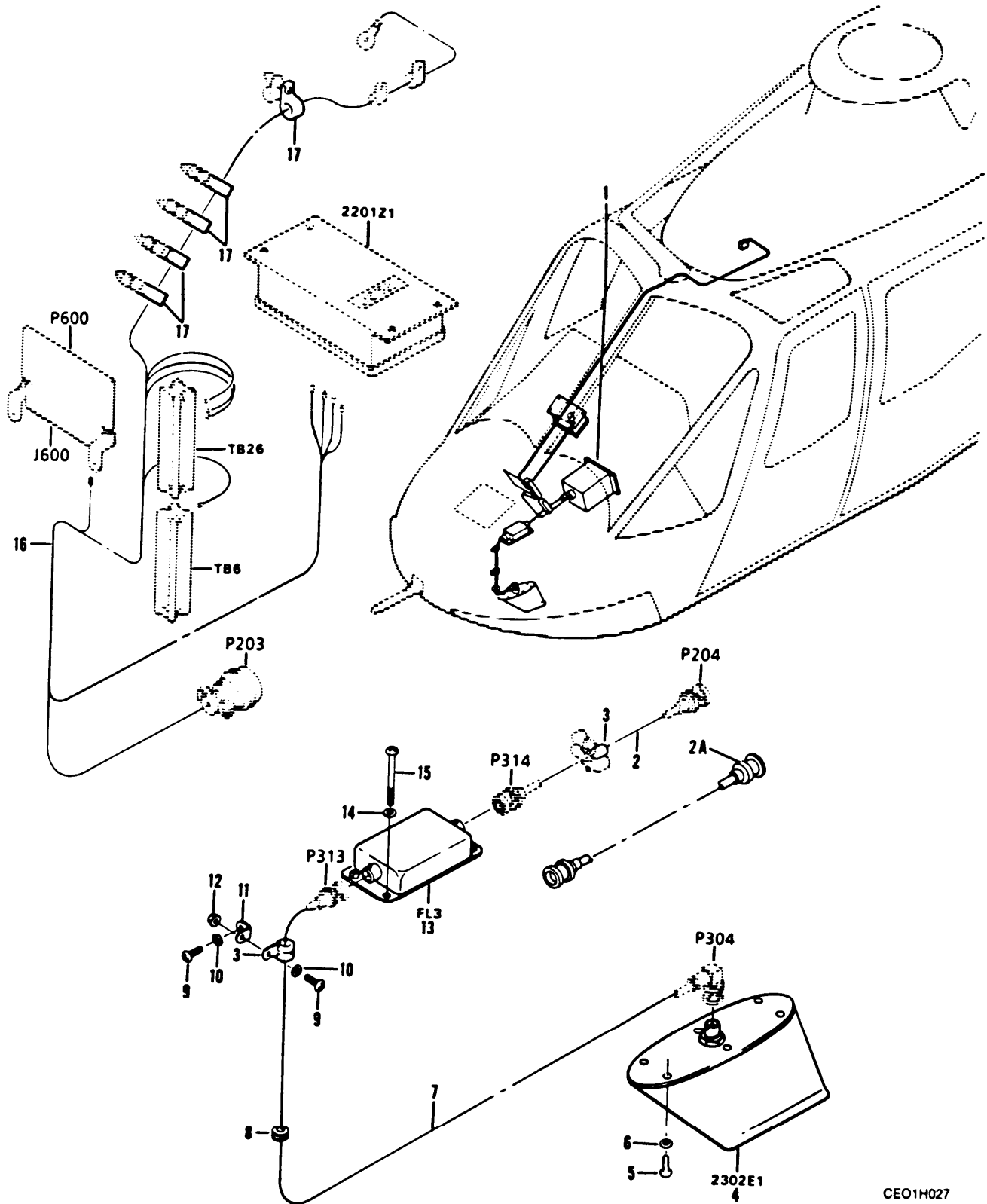
Figure 29. UHF-AM Communications System
