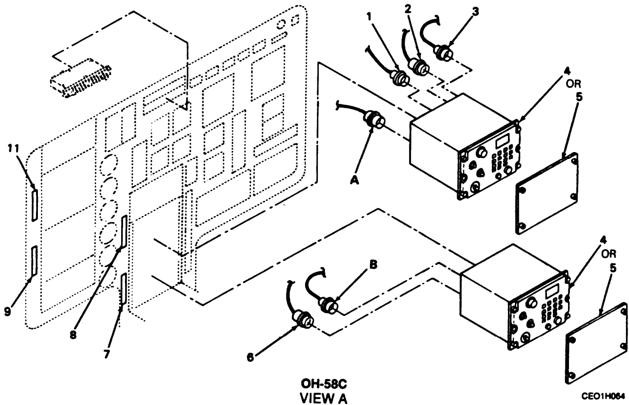
Figure 12. VHF-FM Communications System with SINCGARS, Console (Sheet 2 of 4)
