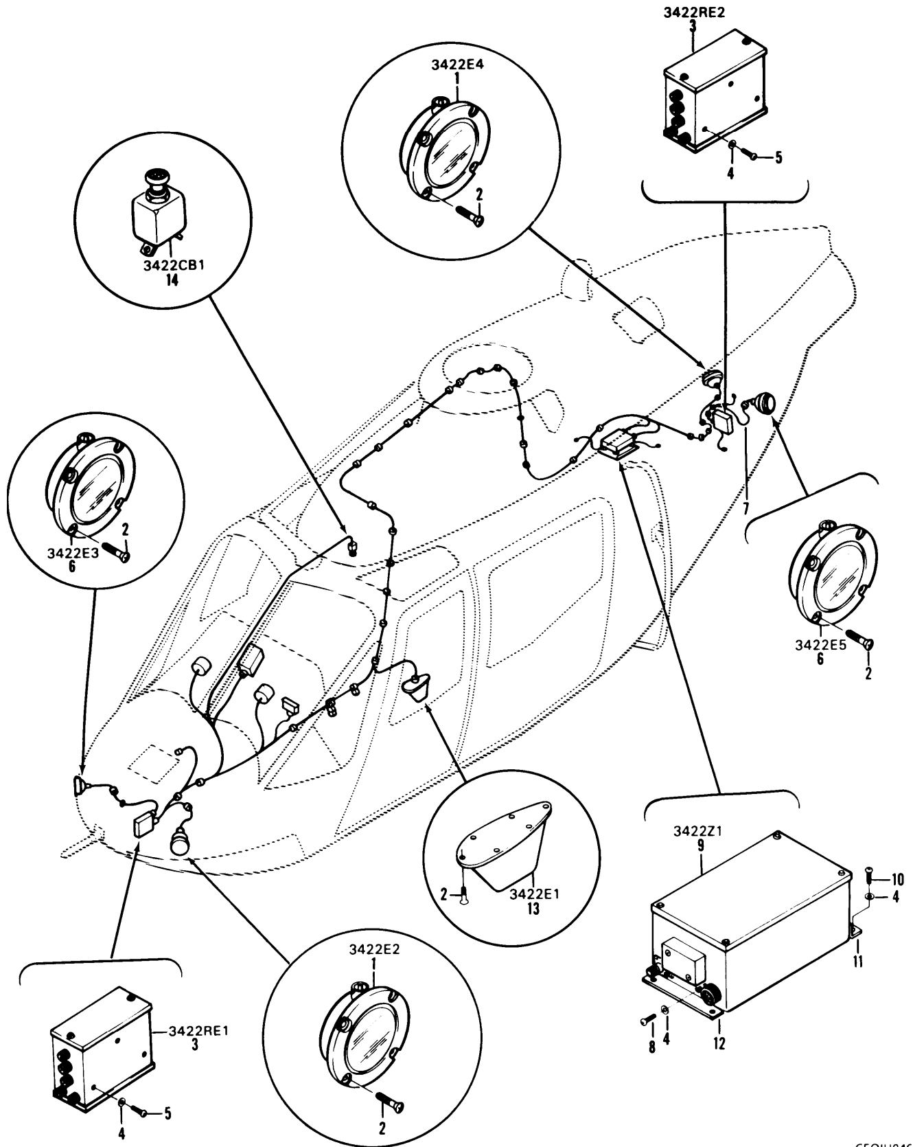
Figure 47. Detecting Set, Radar Signal AN/APR-39(V)1 (C Model Only) (Sheet 1 of 5).
