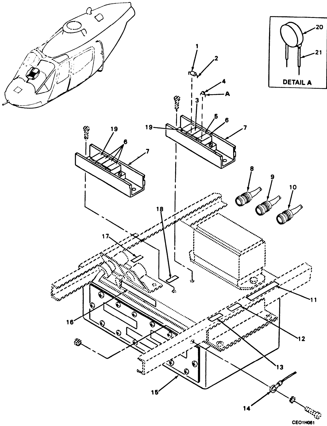
Figure 6. Signal Discriminator, MD-1219/A, DSK-9-03570-501
