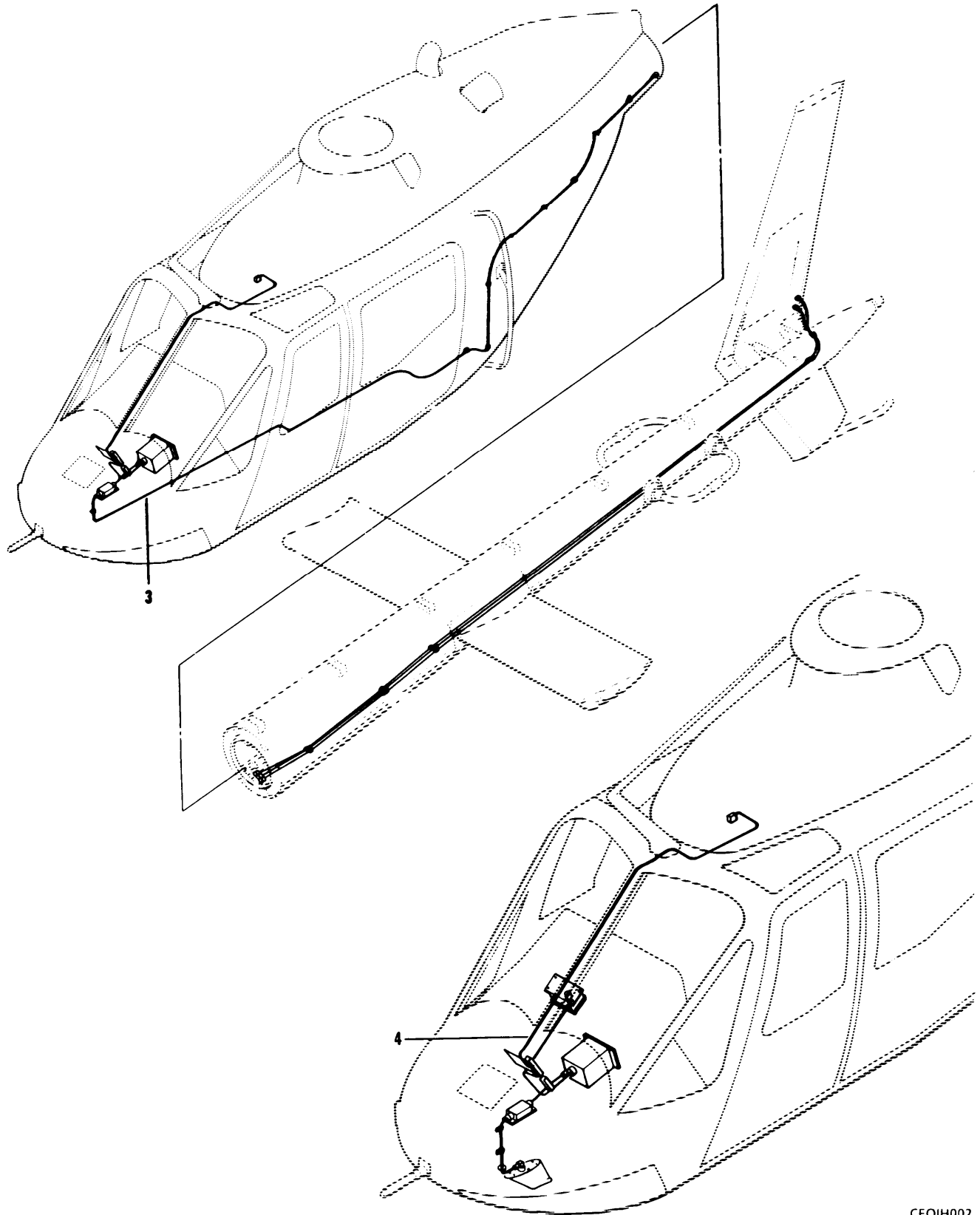
Figure 1. OH-58A/C Electronics Configuration (Sheet 2 of 7).
