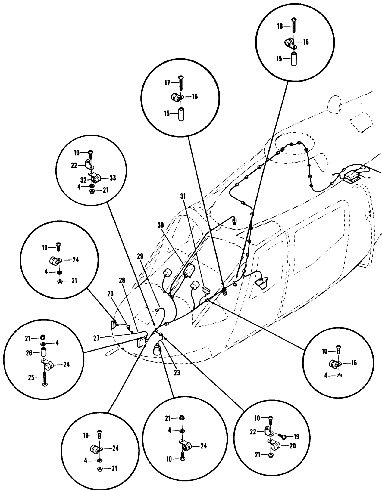
Figure 47. Detecting Set, Radar Signal AN/APR-39(V)1 (C Model Only) (Sheet 2 of 5).
