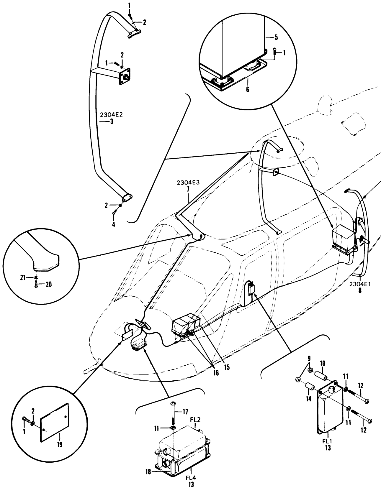
Figure 11. VHF-FM Communications System (Sheet 1 of 3).
