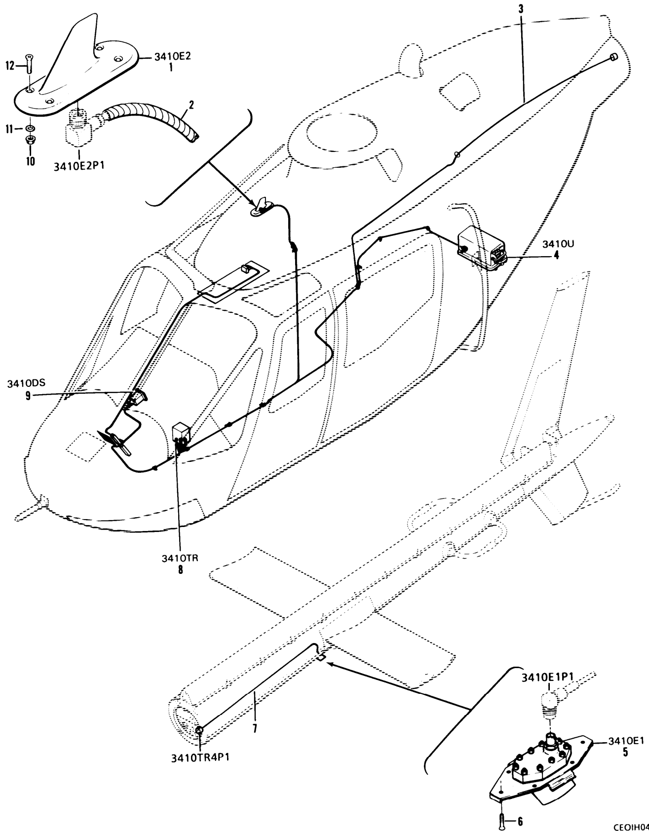
Figure 43. Transponder (IFF) System AN/APX-100 (C Model only) (Sheet 1 of 2).
