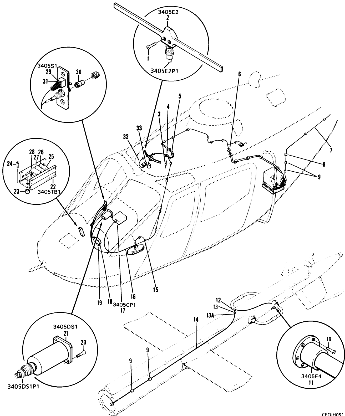
Figure 49. Civil Navigation System AN/ARN-123(V)/1 (C Model Only) (Sheet 1 of 3).
