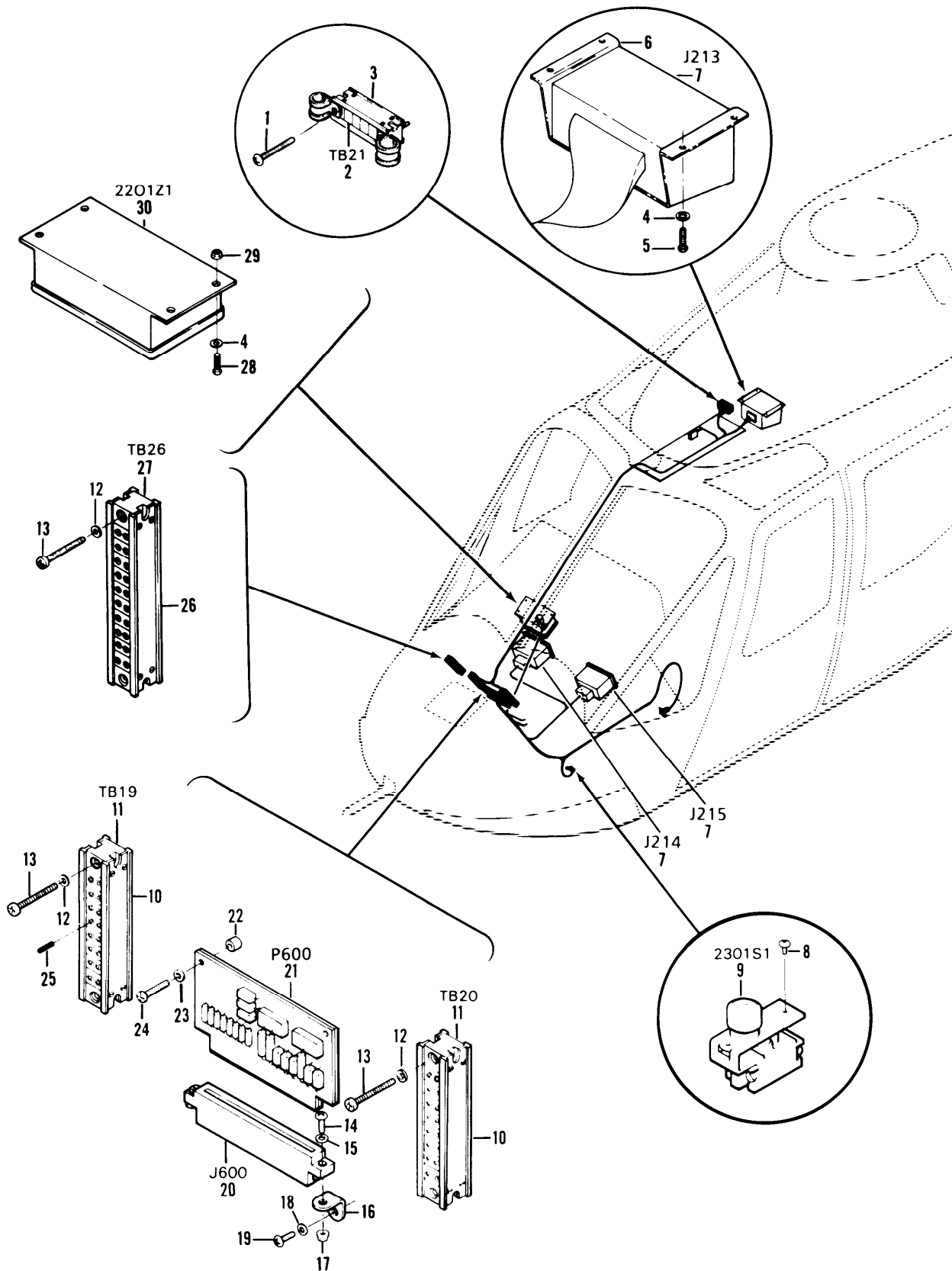
Figure 2. Intercom System (Sheet 1 of 3).
