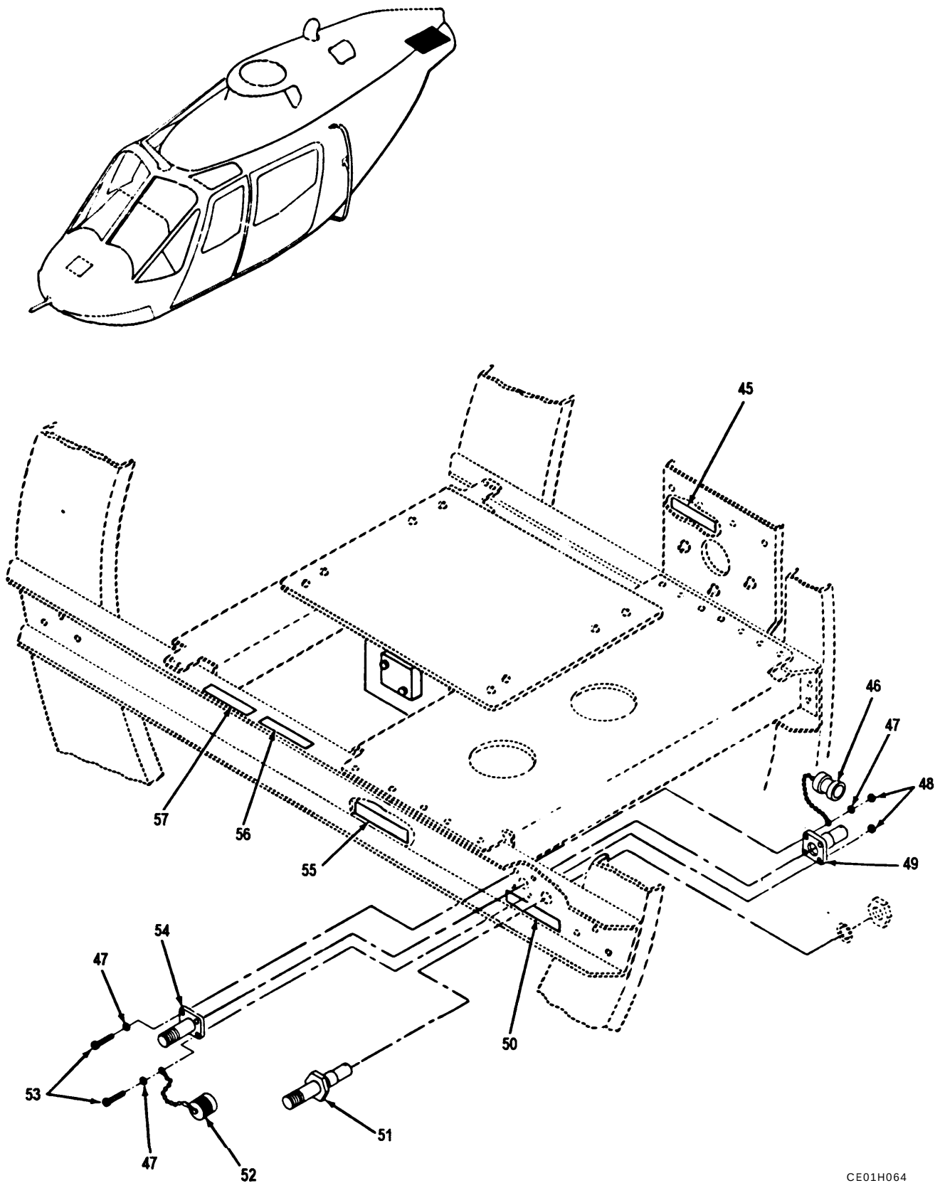
Figure 47. Detecting Set, Radar Signal AN/APR-39(V)1 (C Model Only) (Sheet 5 of 5).
