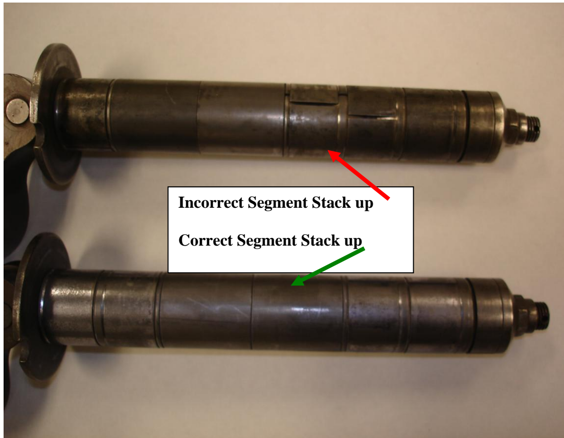
Figure 1: Example of incorrect and correct stack up showing MR Blade Expandable Bolt, PN 406-310-103-103.
